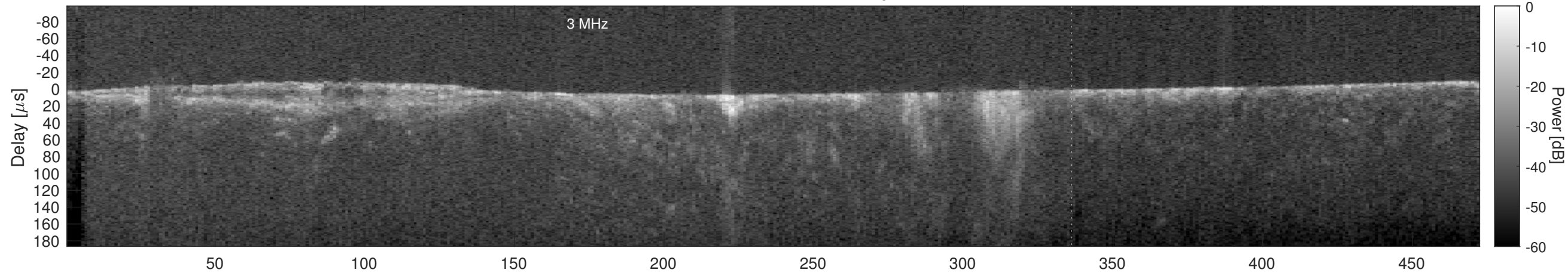
Orbit 13729, Cluttergram
