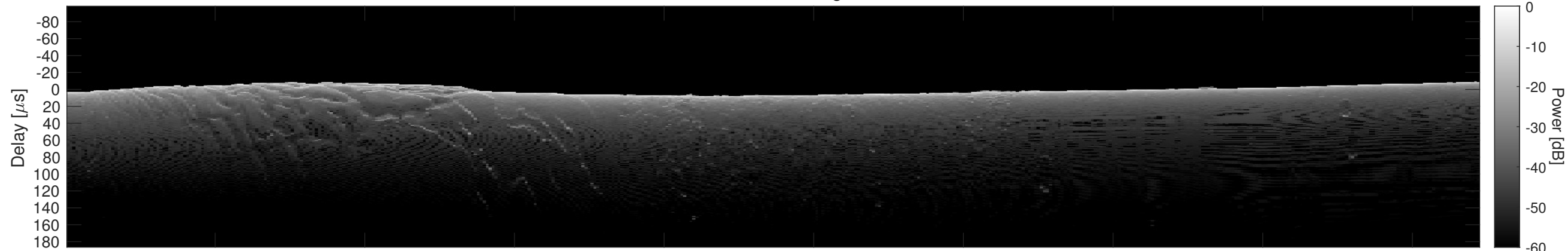
Orbit 13729, Cluttergram
