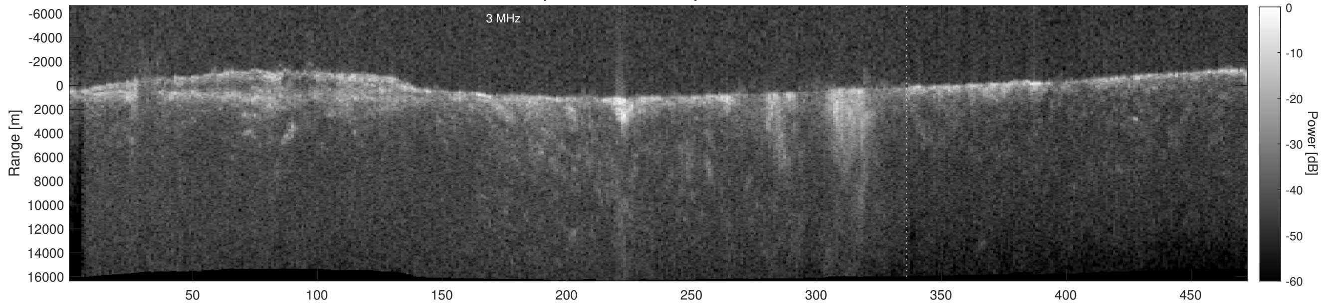
Orbit 13729, Depth-Corrected Cluttergram
