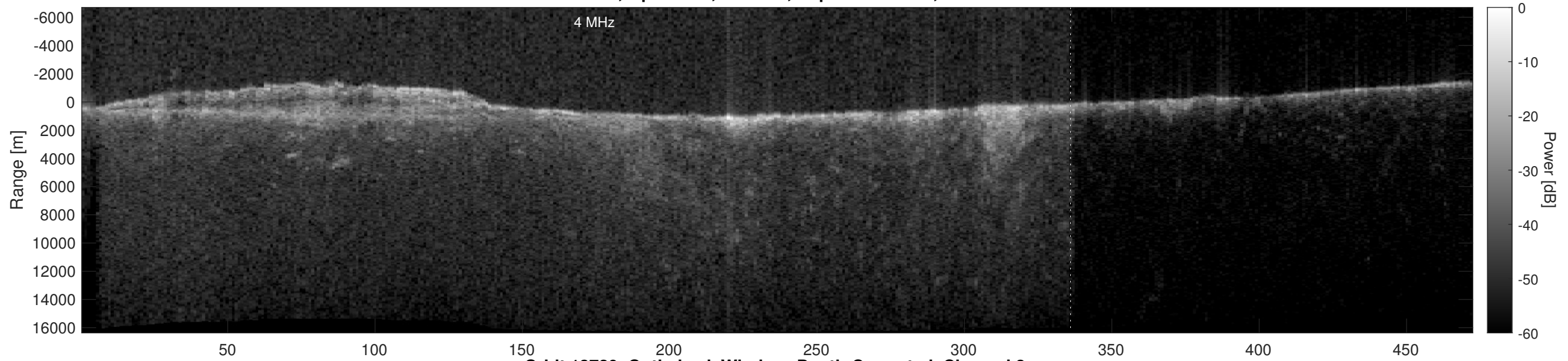
Orbit 13729, Optimized, Window, Depth-Corrected, Channel 2
