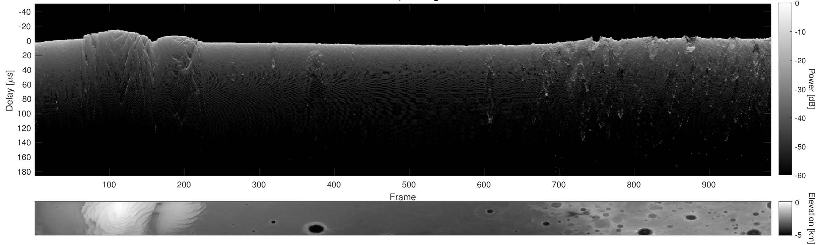
Orbit 13742, Cluttergram
