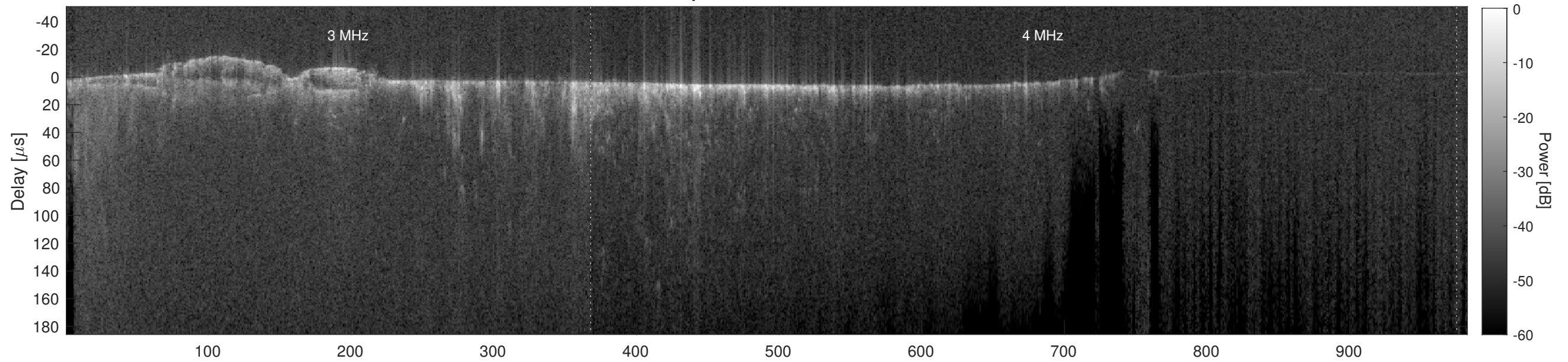
Orbit 13742, Cluttergram
