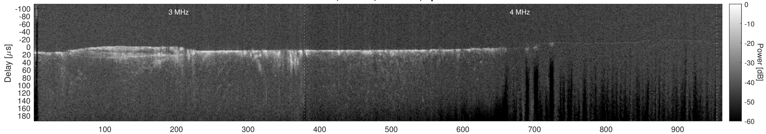
Orbit 13752, Cluttergram
