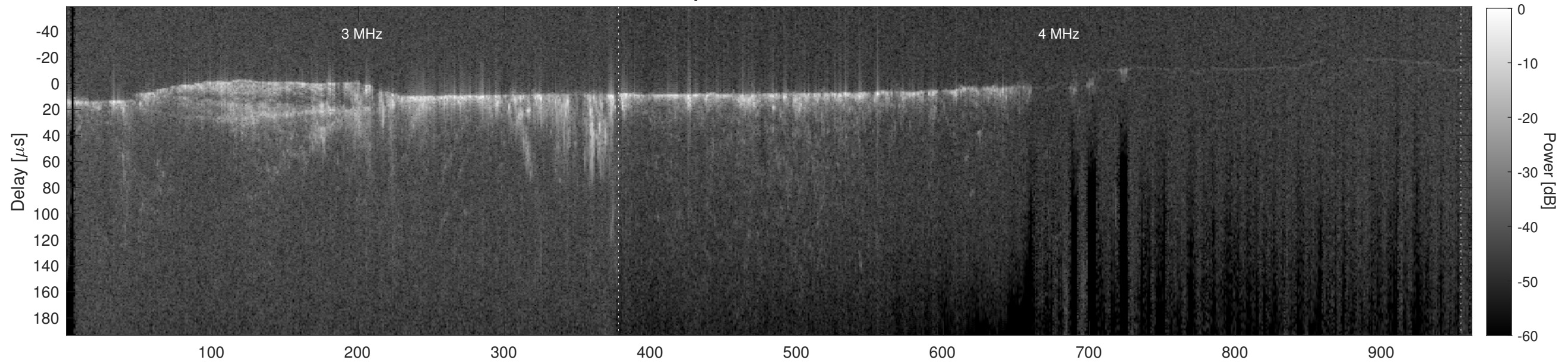
Orbit 13752, Cluttergram
