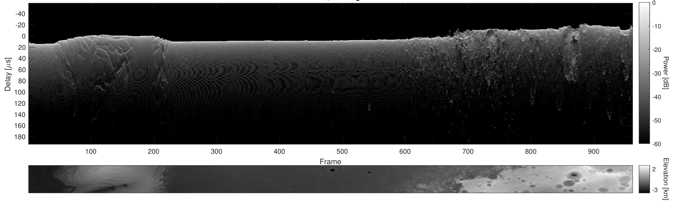
Orbit 13752, Cluttergram
