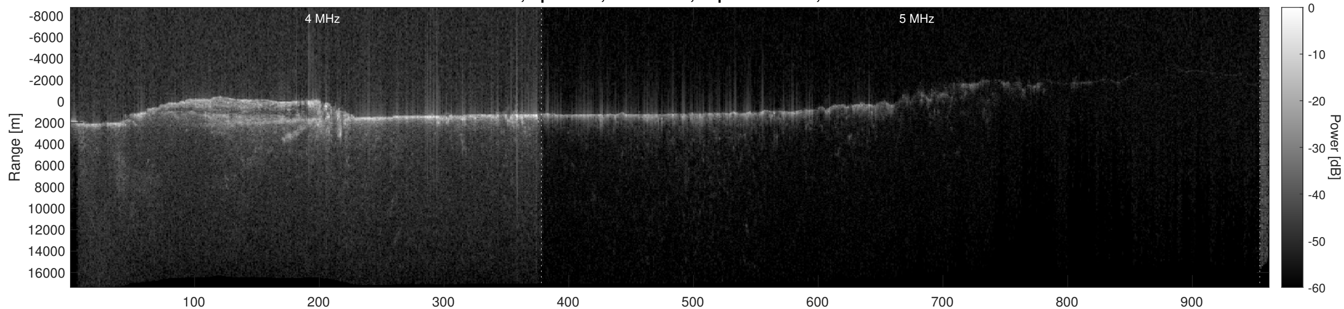
Orbit 13752, Optimized, No Window, Depth-Corrected, Channel 2
