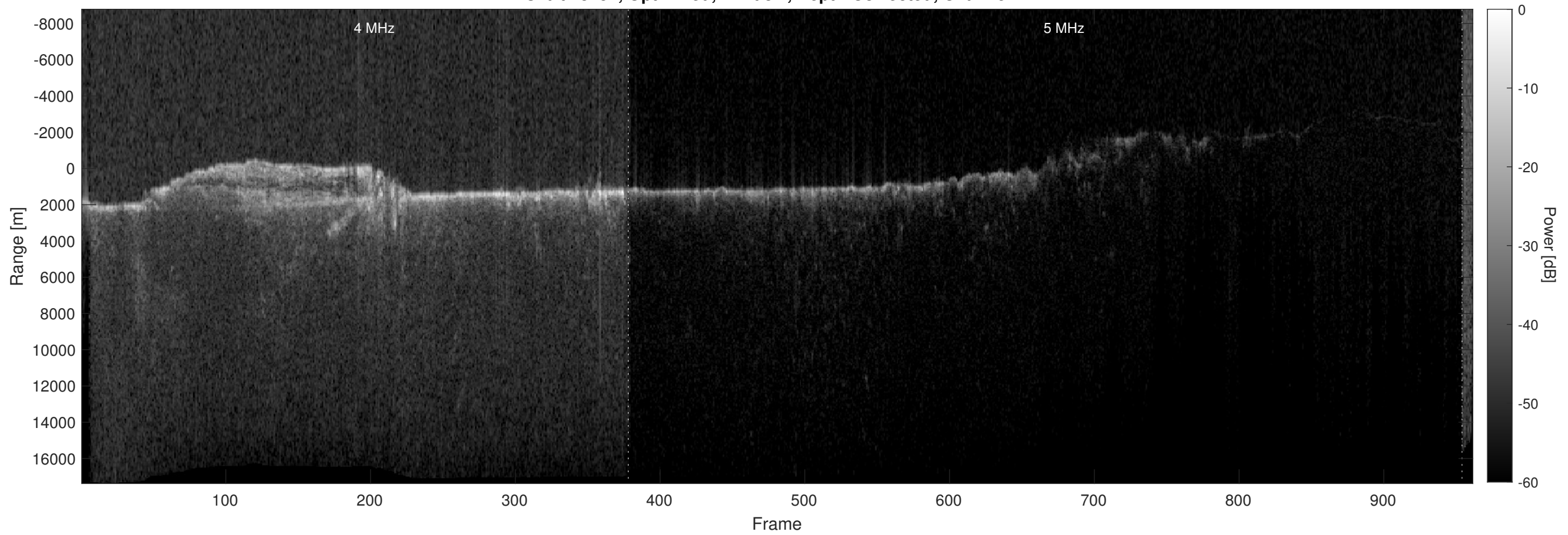
Orbit 13752, Optimized, Window, Depth-Corrected, Channel 2
