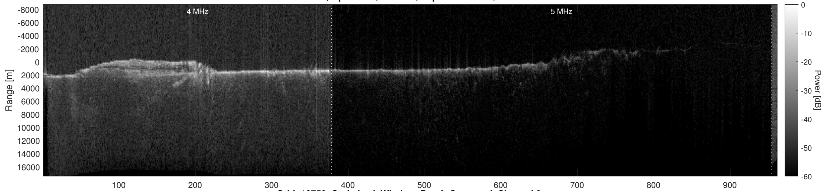
Orbit 13752, Optimized, Window, Depth-Corrected, Channel 2
