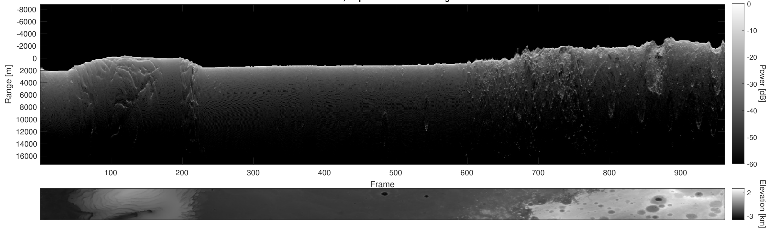
Orbit 13752, Depth-Corrected Cluttergram
