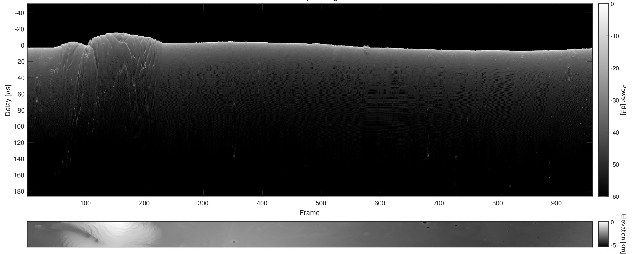
Orbit 13762, Cluttergram
