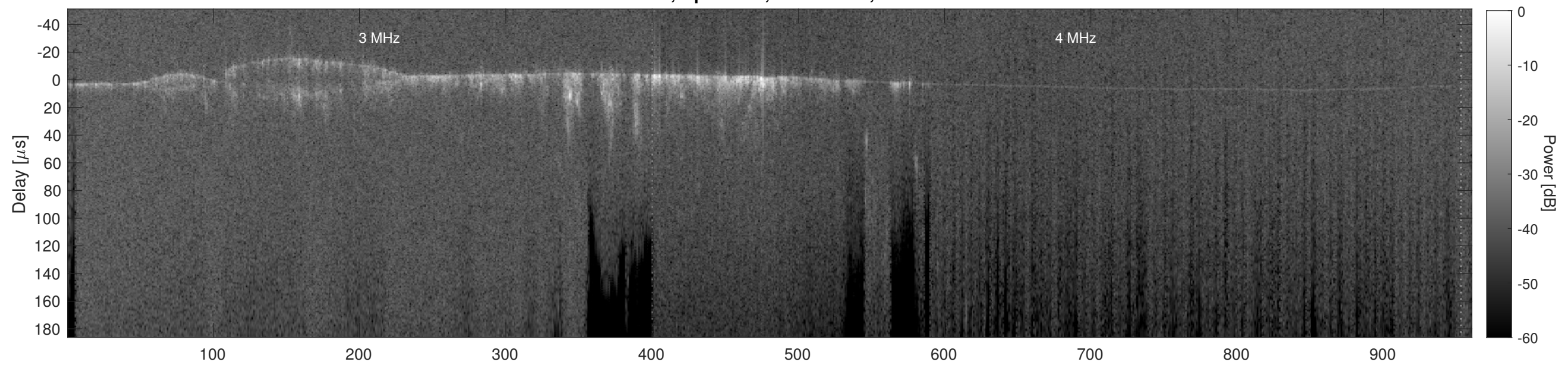
Orbit 13762, Cluttergram
