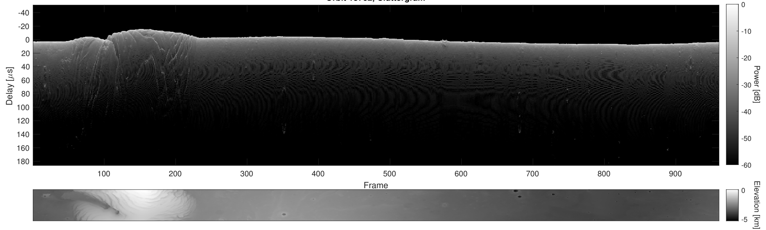
Orbit 13762, Cluttergram
