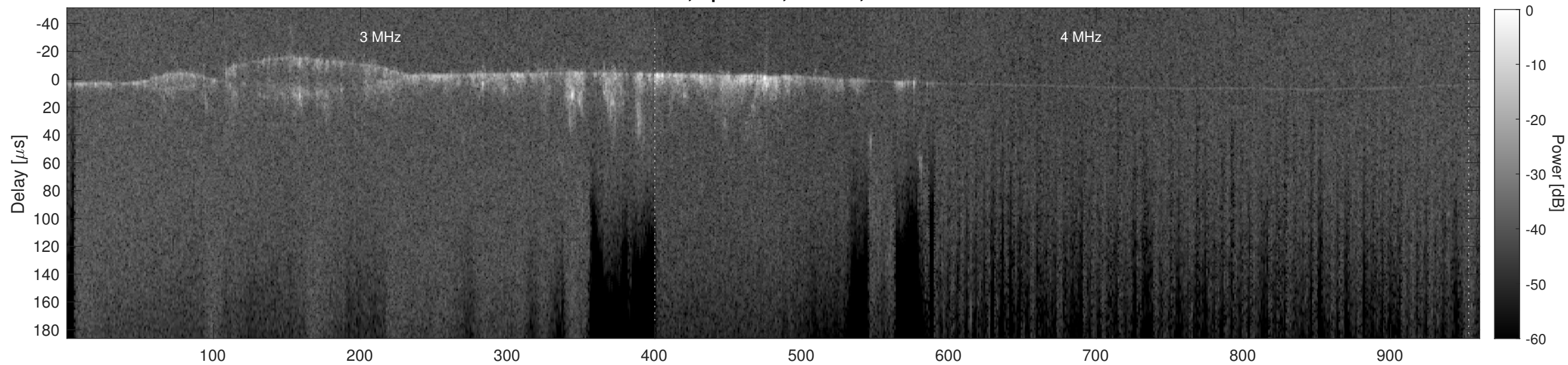
Orbit 13762, Cluttergram
