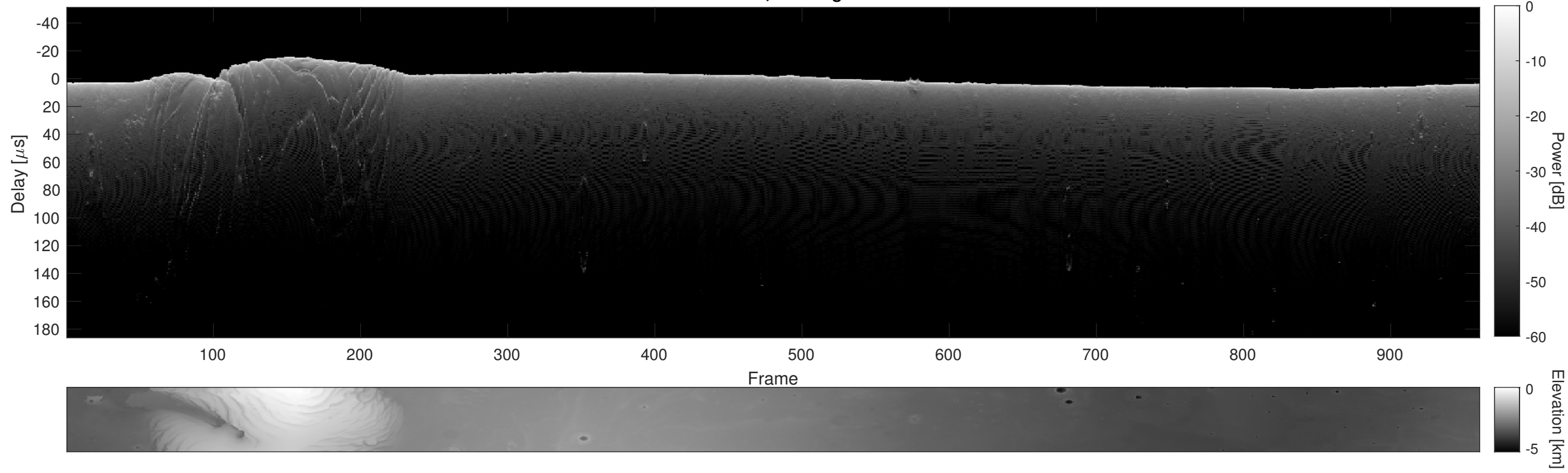
Orbit 13762, Cluttergram
