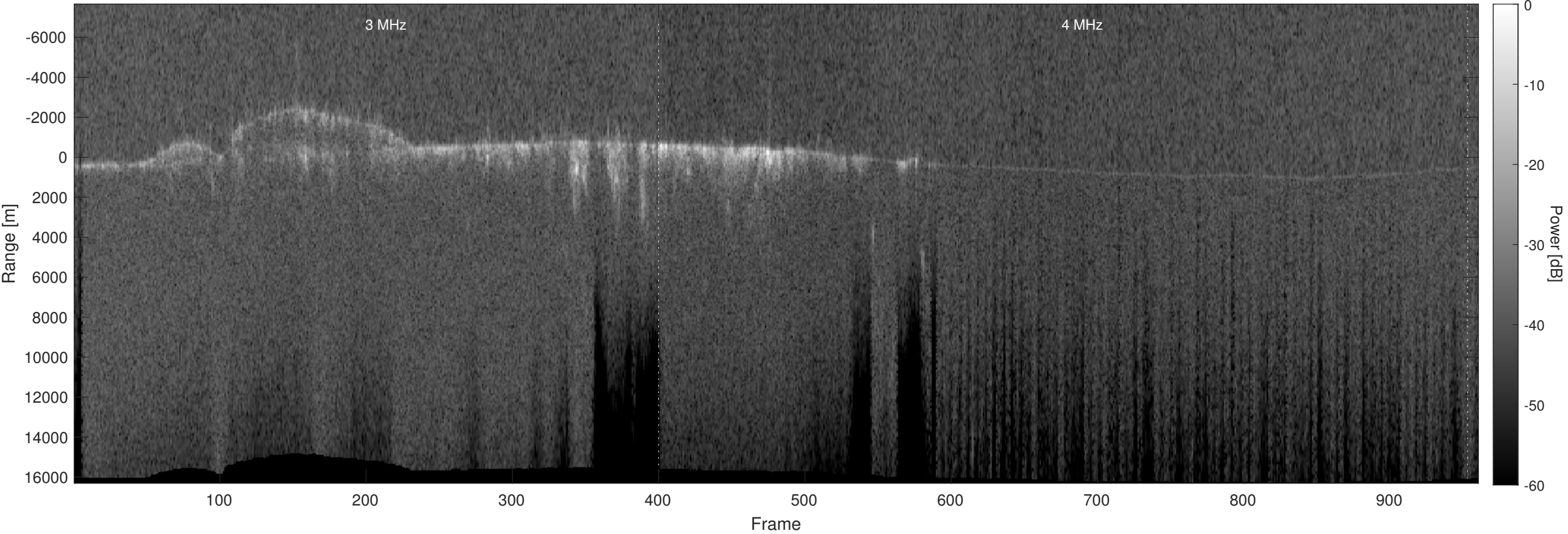
Orbit 13762, Optimized, Window, Depth-Corrected, Channel 2
