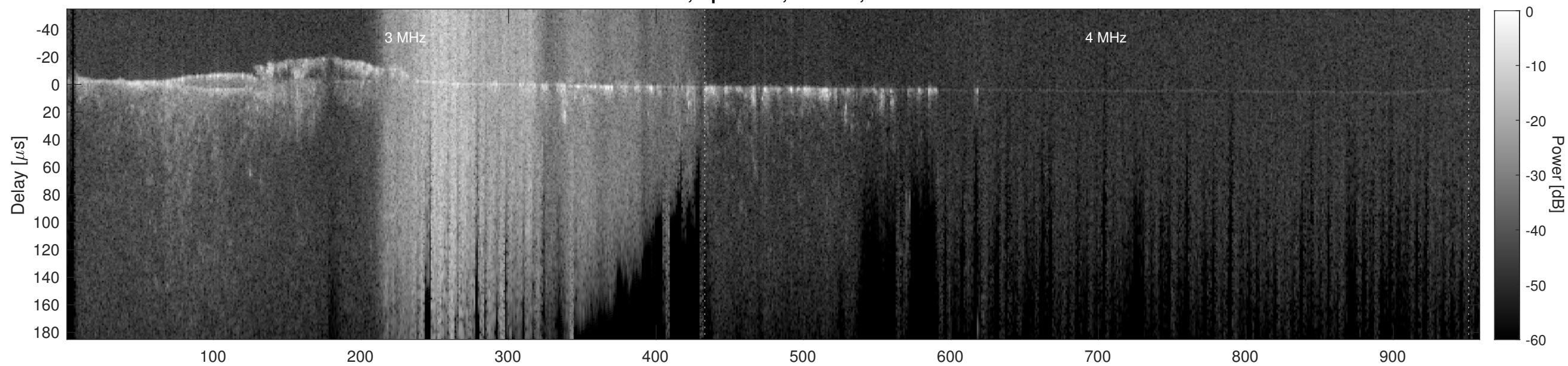
Orbit 13774, Cluttergram
