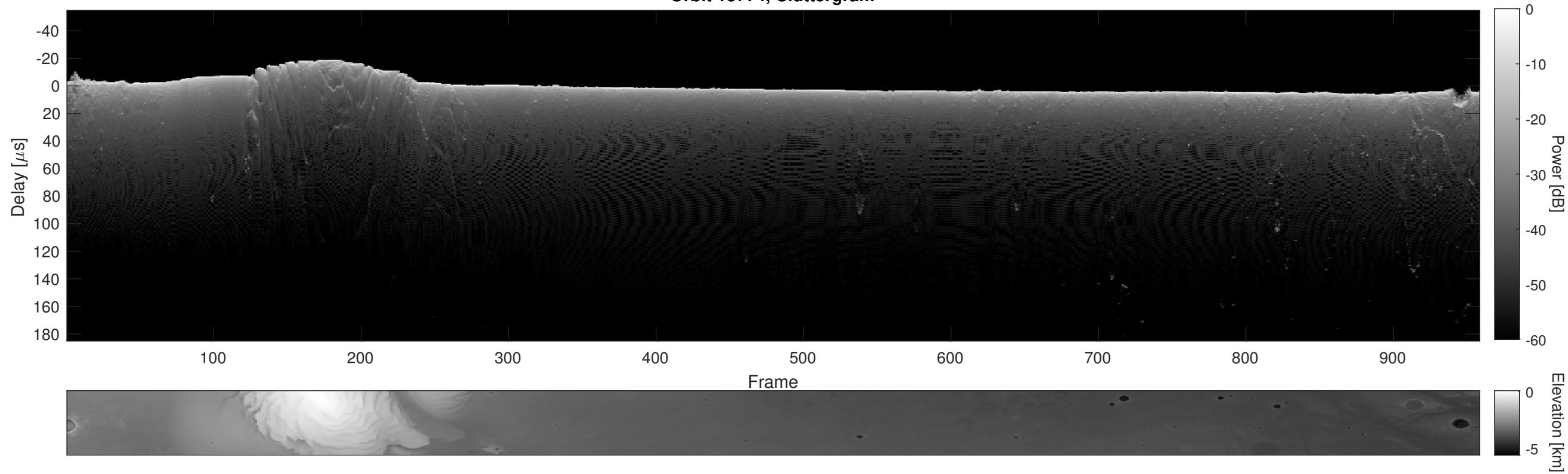
Orbit 13774, Cluttergram
