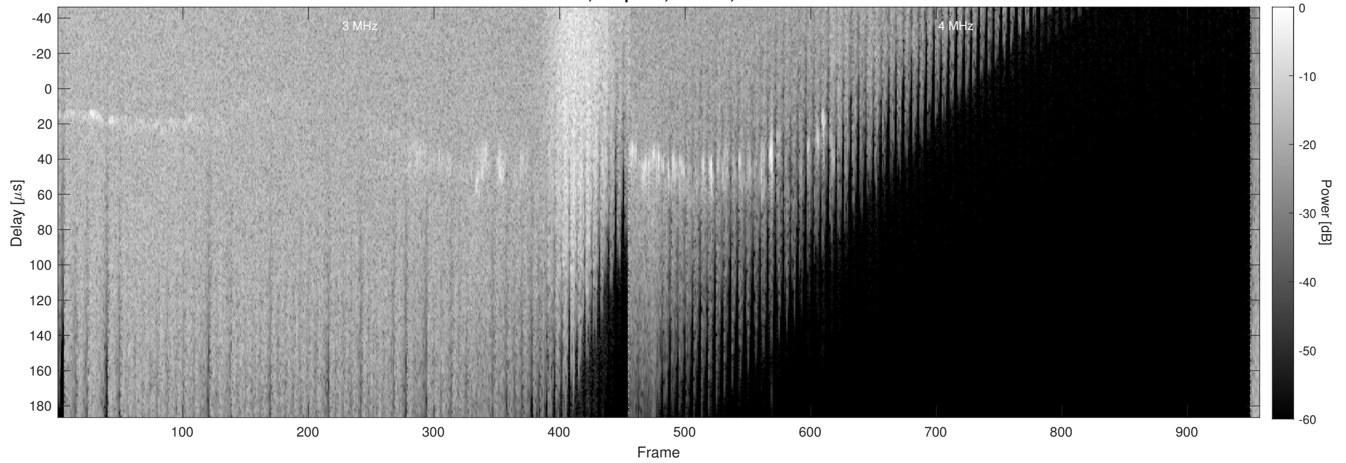
Orbit 13784, Chapman, Window, Channel 2
