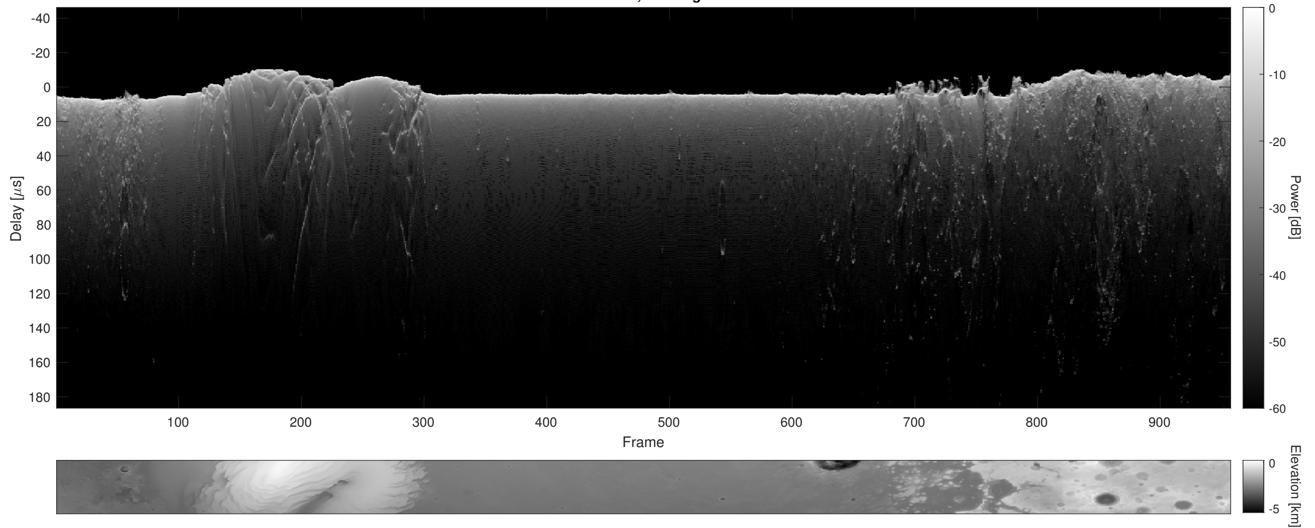
Orbit 13784, Cluttergram
