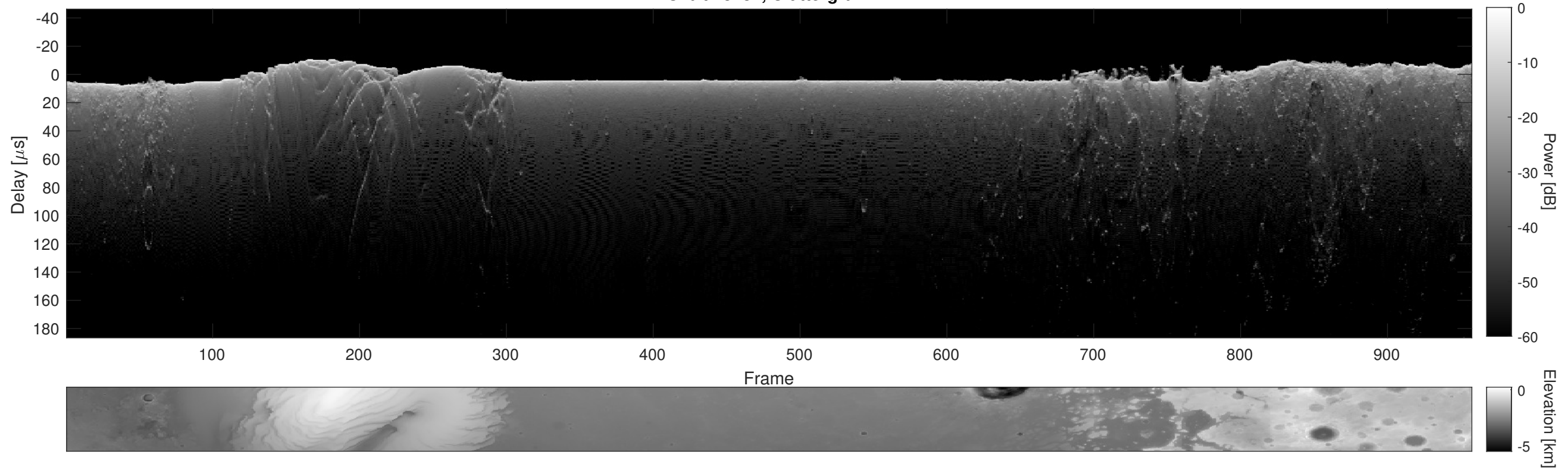
Orbit 13784, Cluttergram
