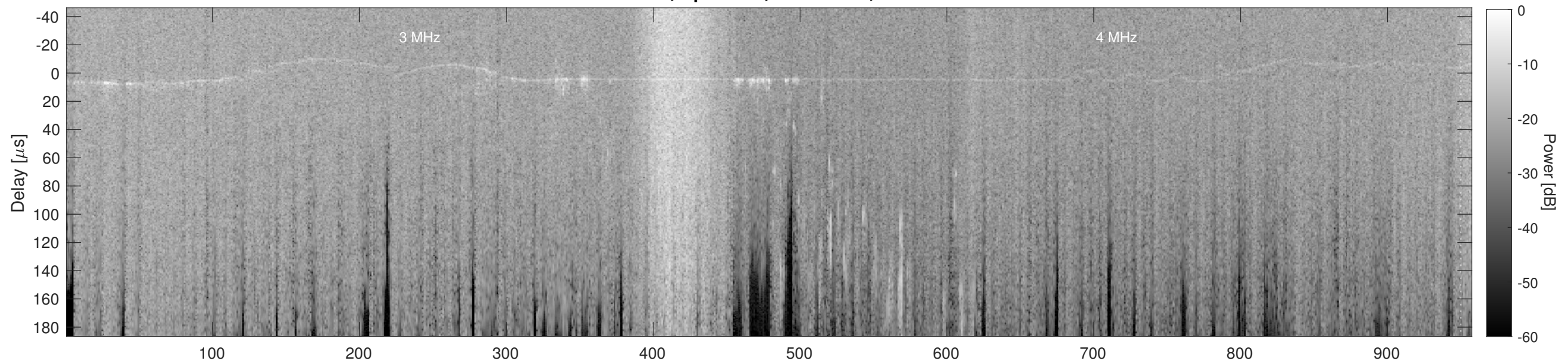
Orbit 13784, Cluttergram
