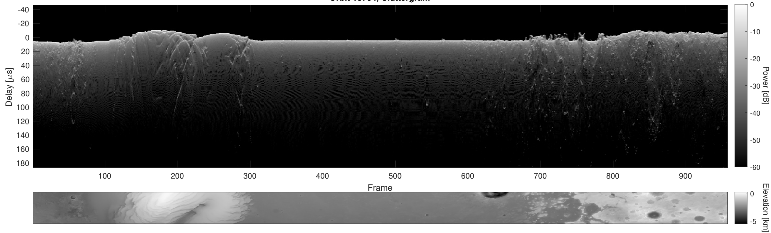
Orbit 13784, Cluttergram
