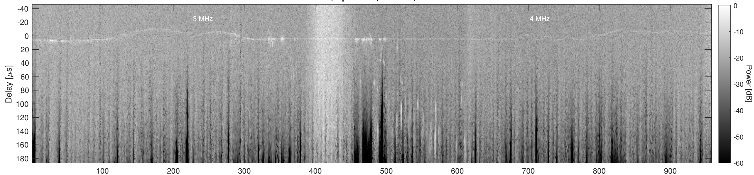
Orbit 13784, Cluttergram
