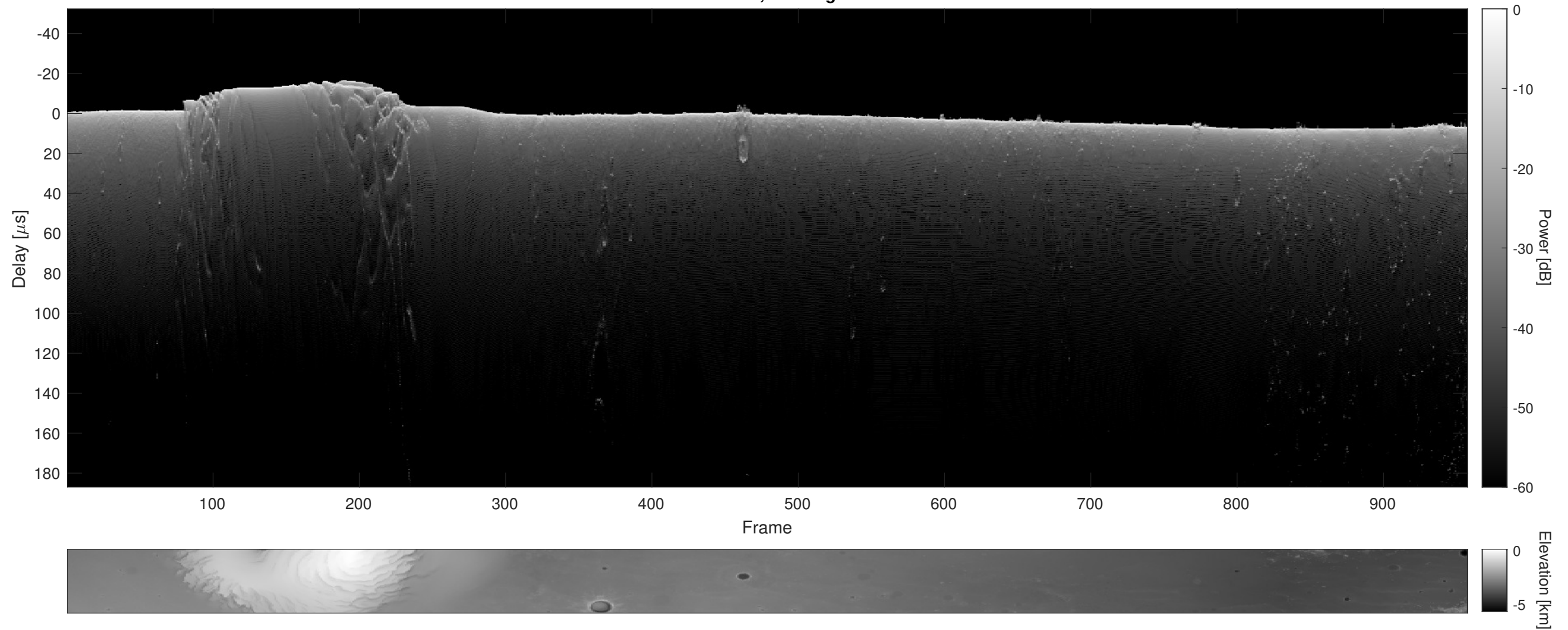
Orbit 13786, Cluttergram
