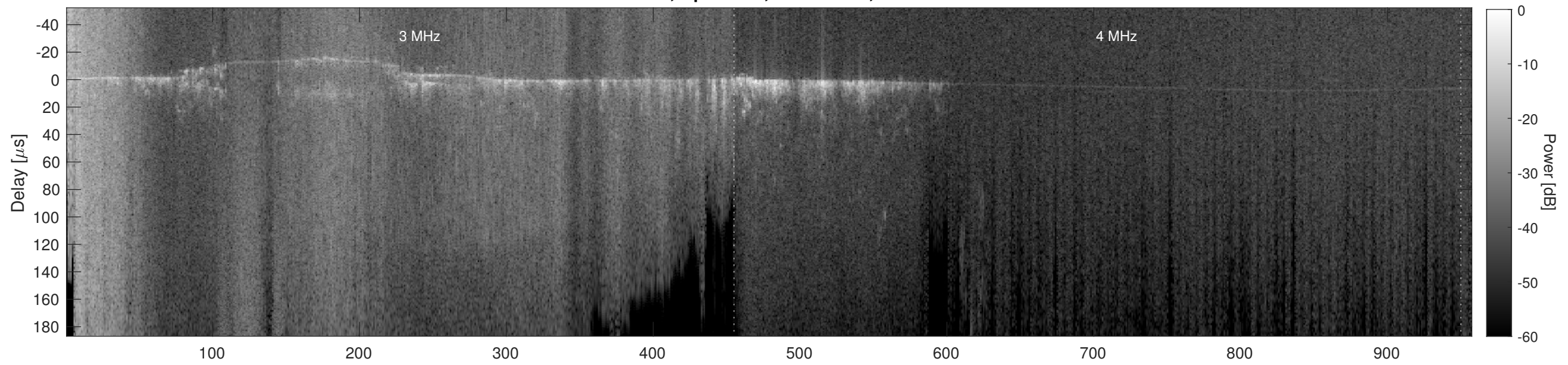
Orbit 13786, Cluttergram
