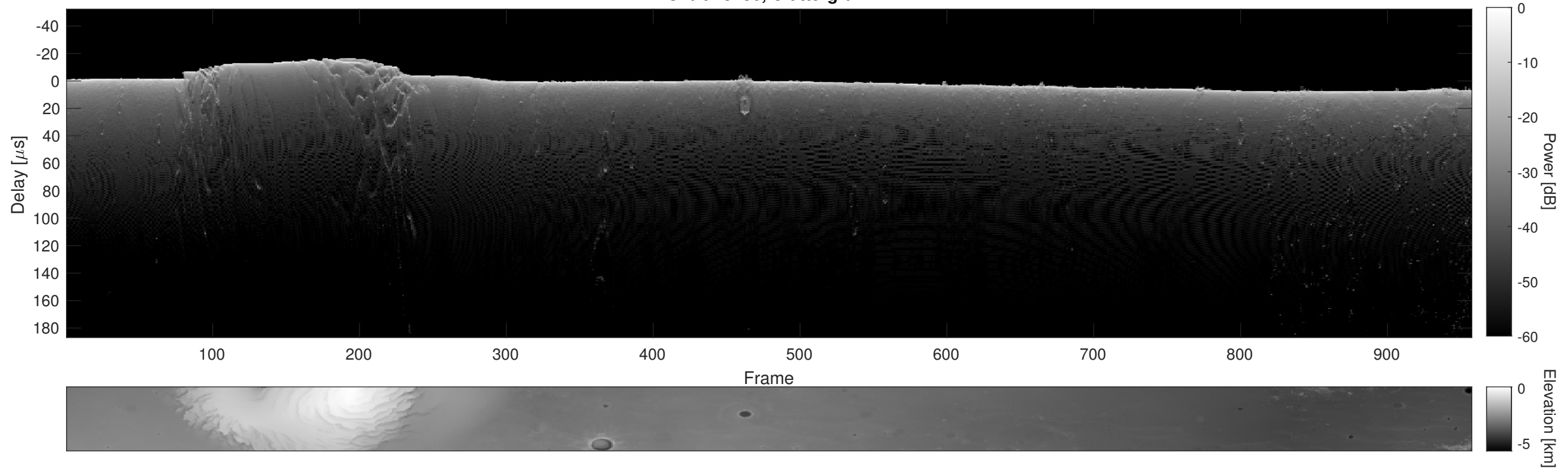
Orbit 13786, Cluttergram
