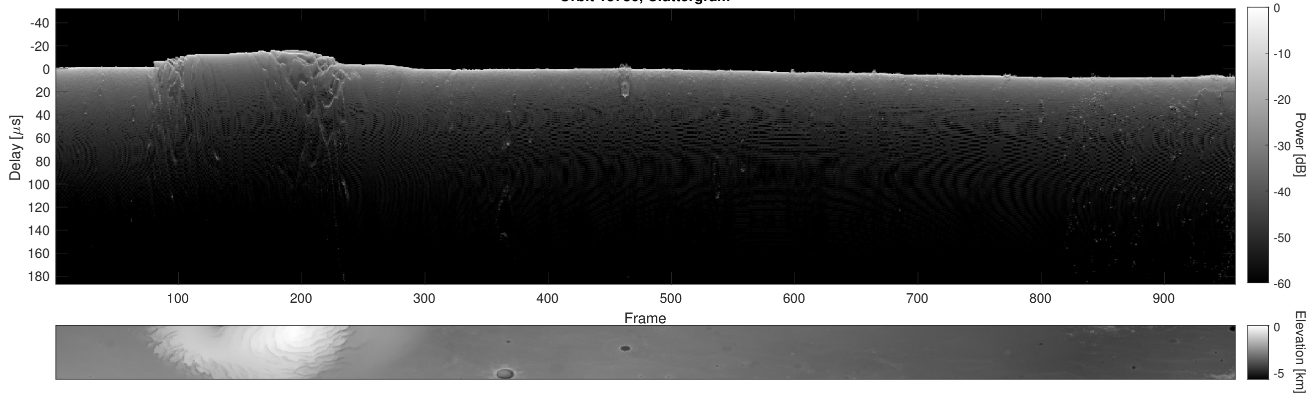
Orbit 13786, Cluttergram
