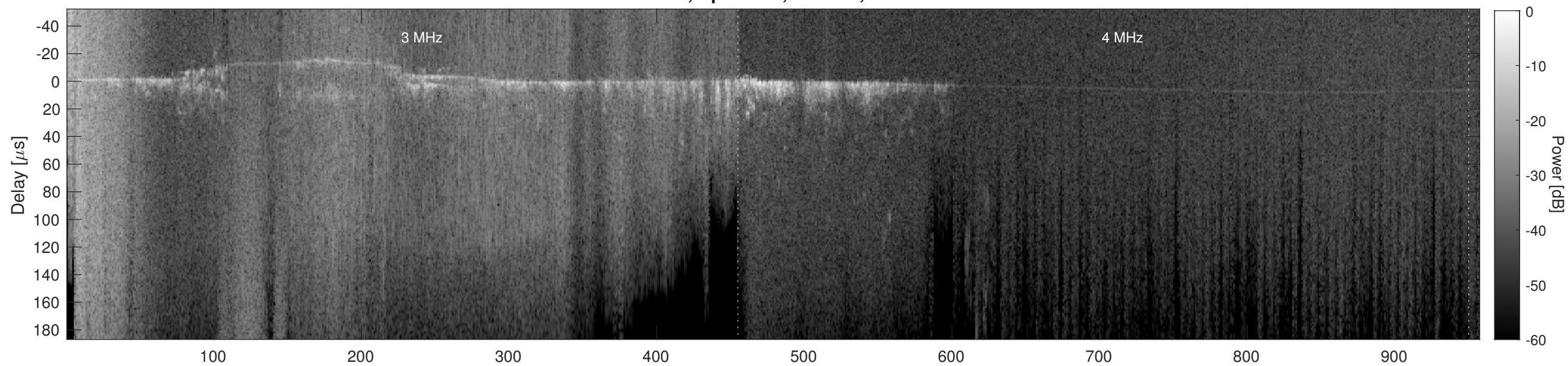
Orbit 13786, Cluttergram
