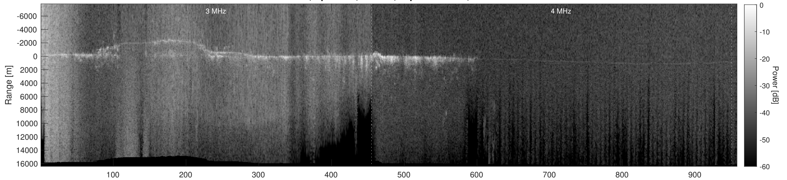
Orbit 13786, Depth-Corrected Cluttergram
