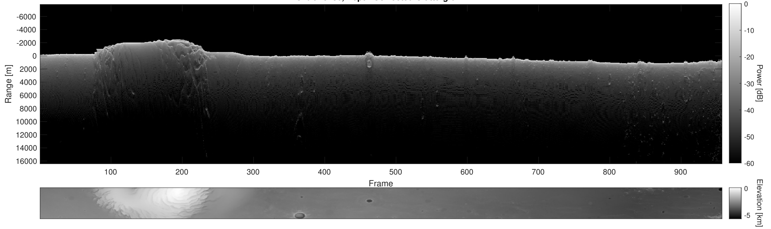
Orbit 13786, Depth-Corrected Cluttergram
