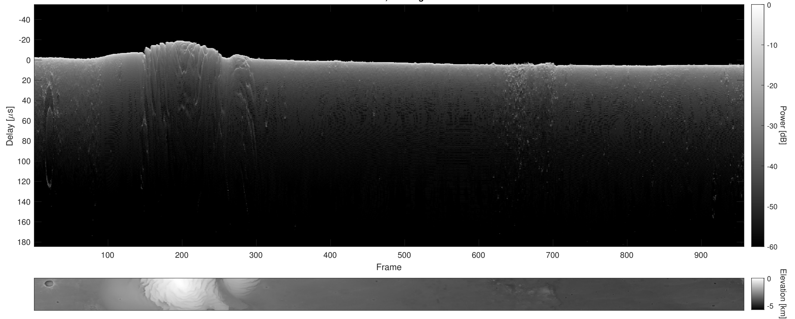
Orbit 13788, Cluttergram
