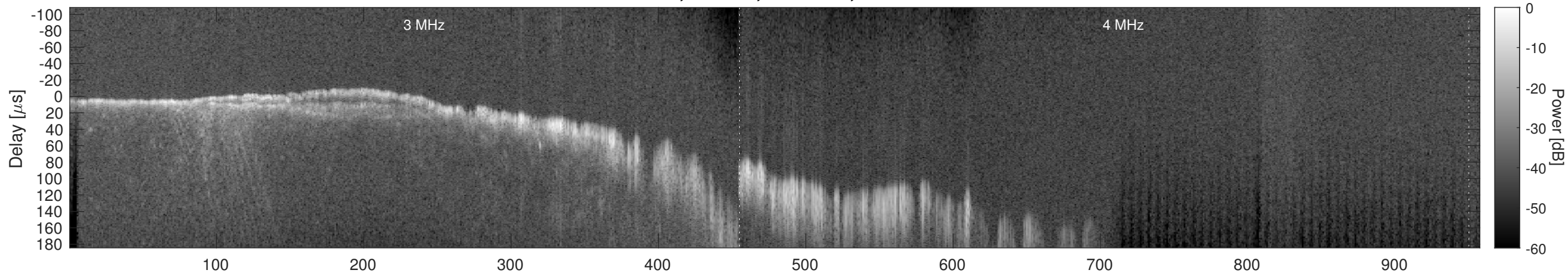
Orbit 13788, Window, Channel 2, Chapman
