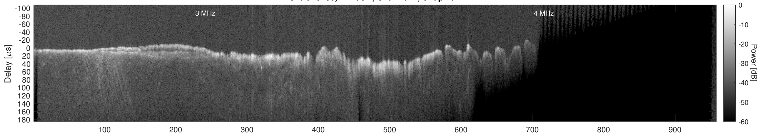
Orbit 13788, Window, Channel 2, Optimized
