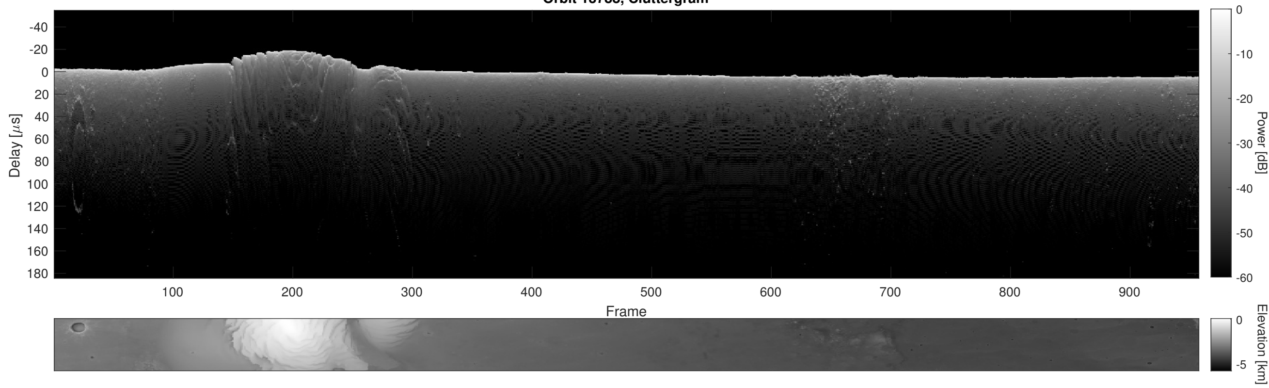
Orbit 13788, Cluttergram
