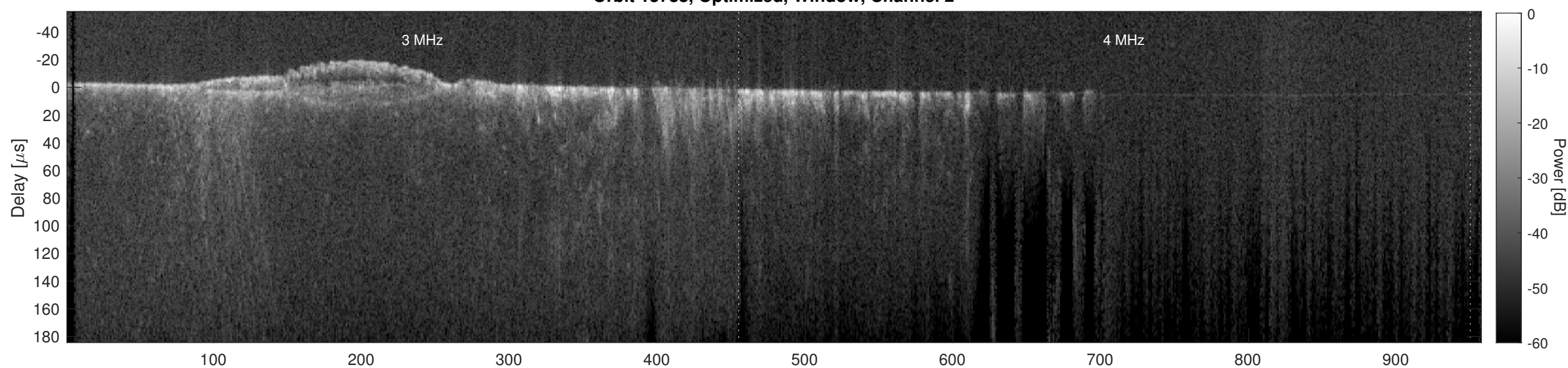
Orbit 13788, Cluttergram
