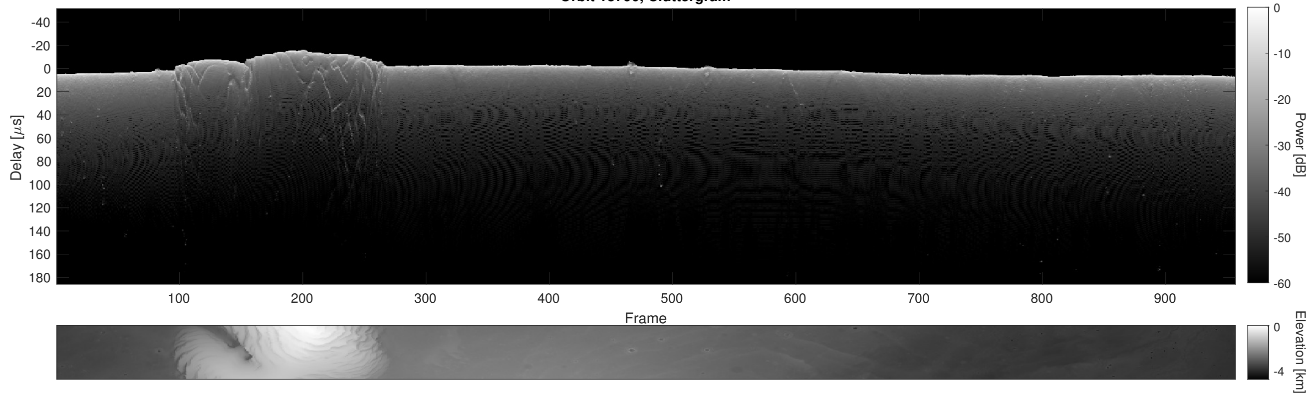
Orbit 13790, Cluttergram
