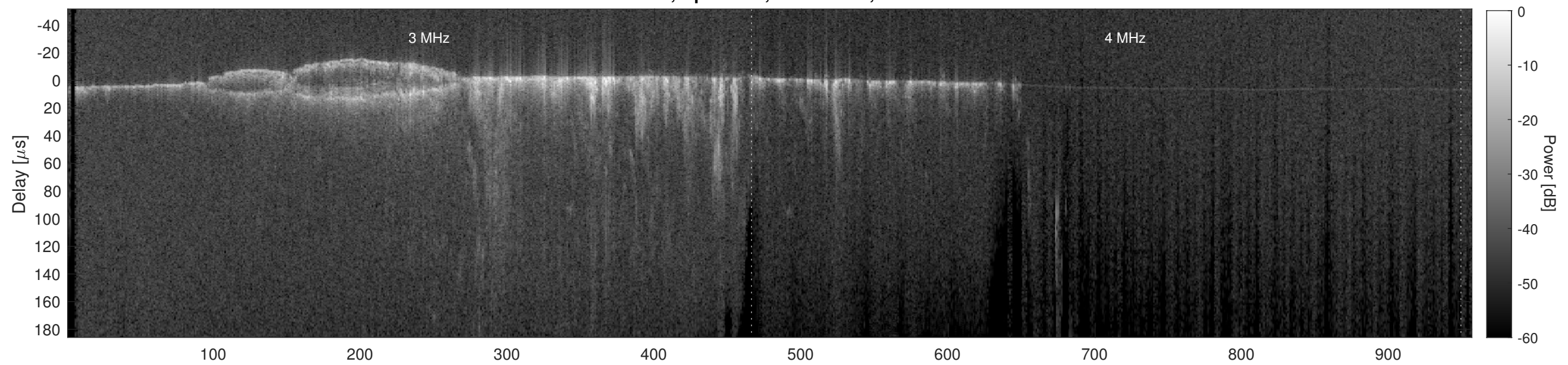
Orbit 13790, Cluttergram
