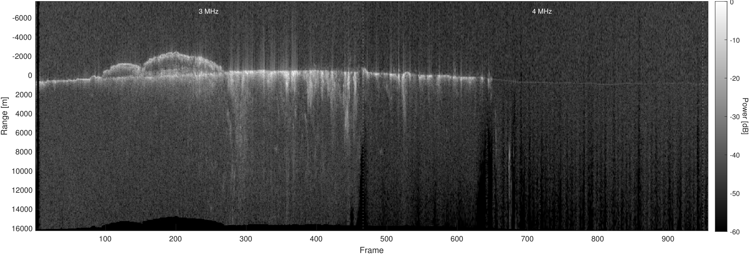
Orbit 13790, Optimized, No Window, Depth-Corrected, Channel 2
