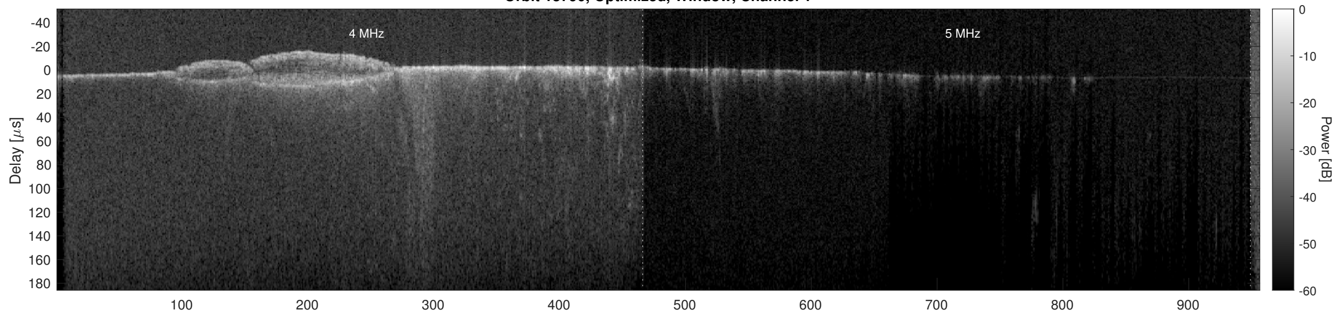
Orbit 13790, Optimized, Window, Channel 2
