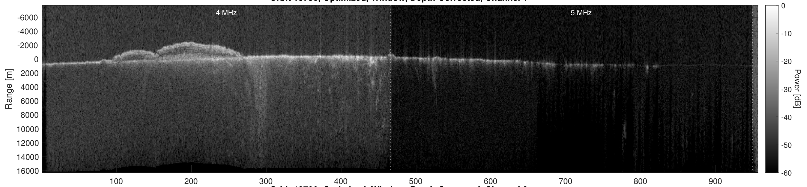
Orbit 13790, Optimized, Window, Depth-Corrected, Channel 2
