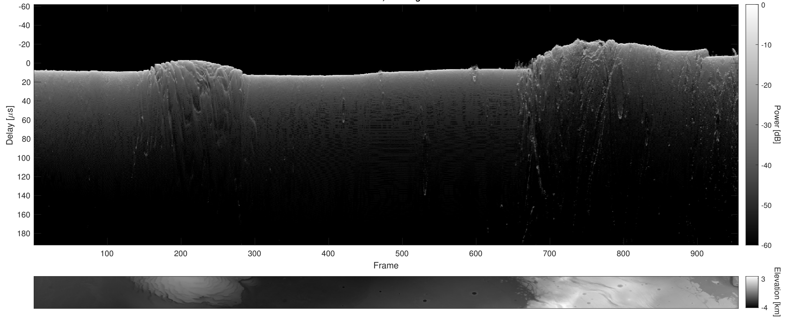
Orbit 13792, Cluttergram
