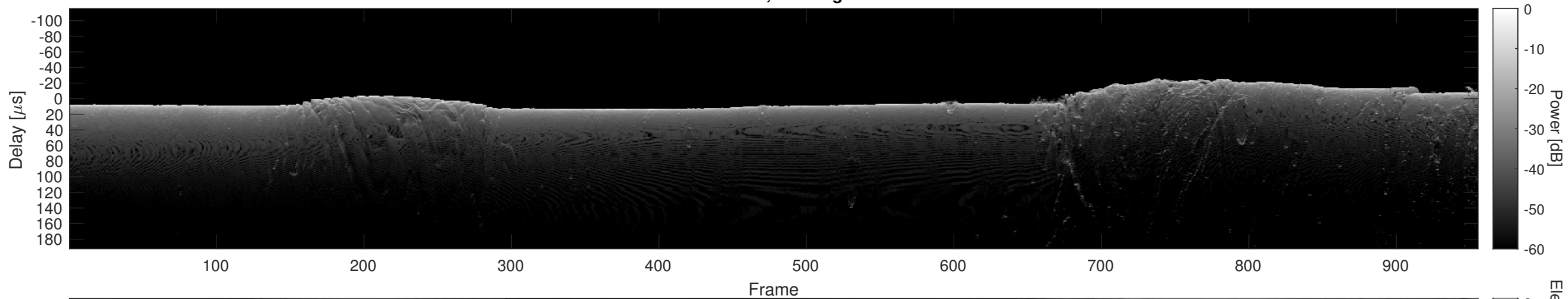
Orbit 13792, Cluttergram
