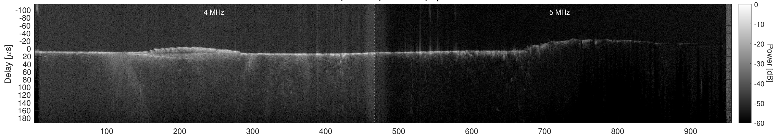
Orbit 13792, Cluttergram
