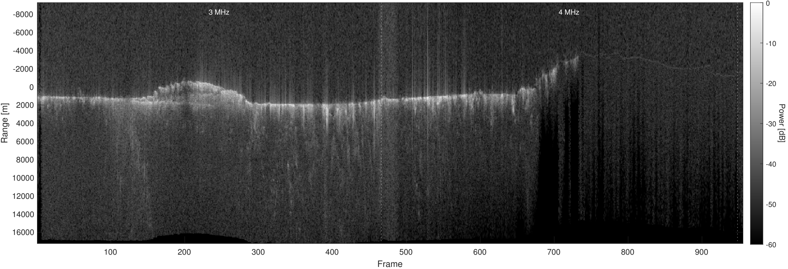
Orbit 13792, Optimized, No Window, Depth-Corrected, Channel 2
