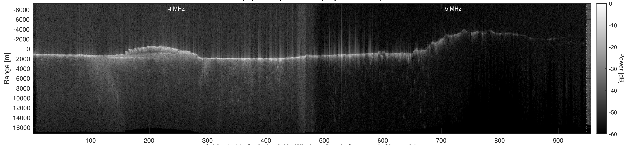
Orbit 13792, Optimized, No Window, Depth-Corrected, Channel 2
