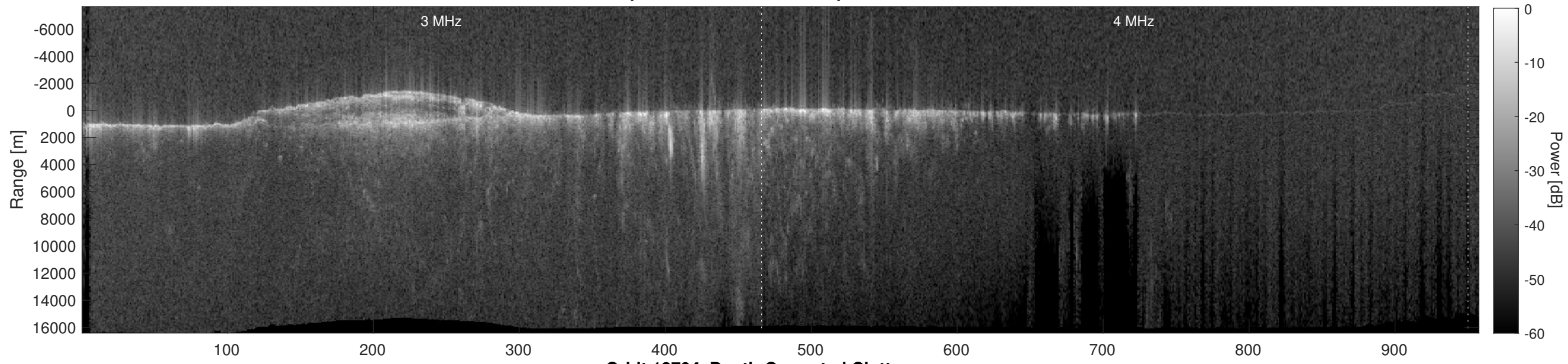
Orbit 13794, Depth-Corrected Cluttergram
