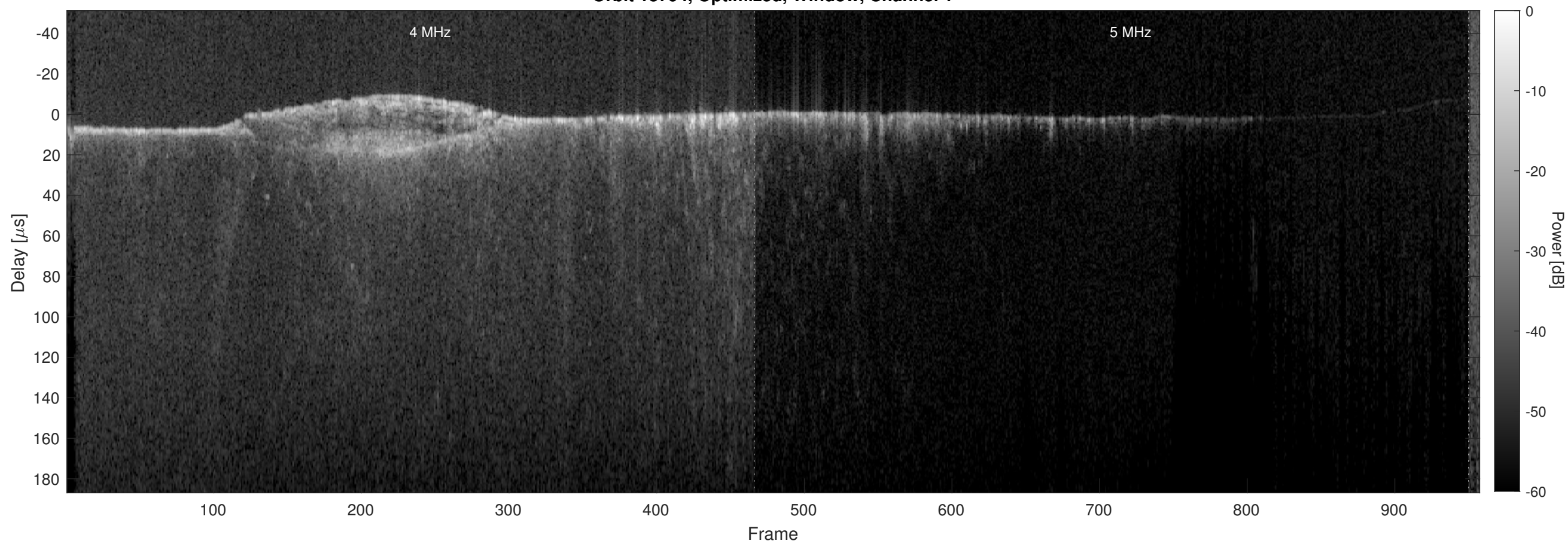
Orbit 13794, Optimized, Window, Channel 2
