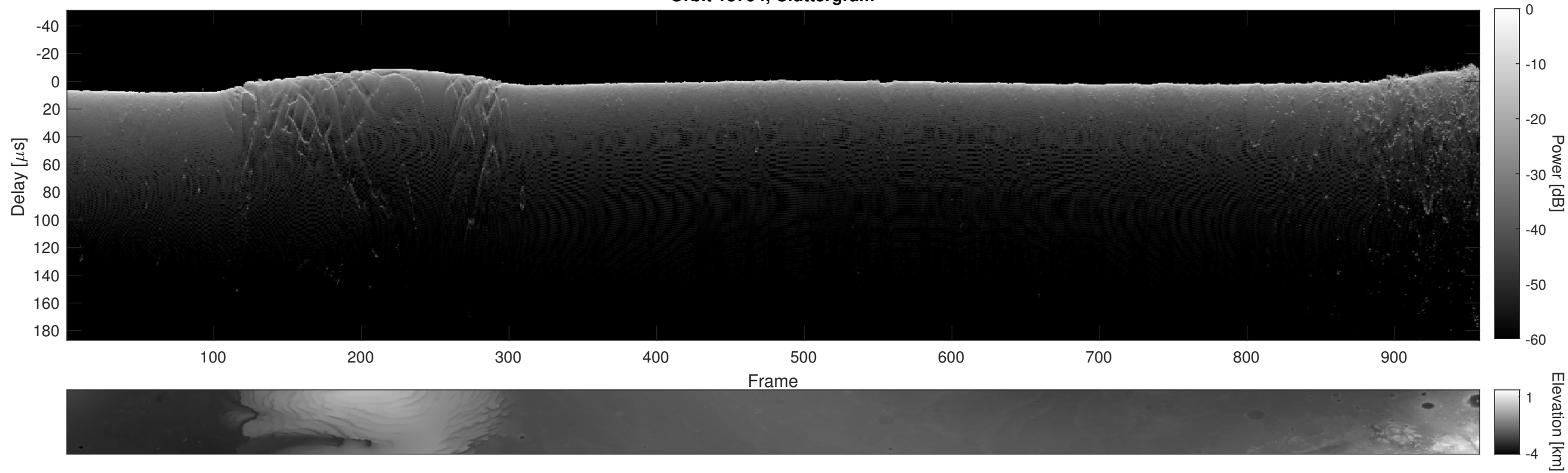
Orbit 13794, Cluttergram
