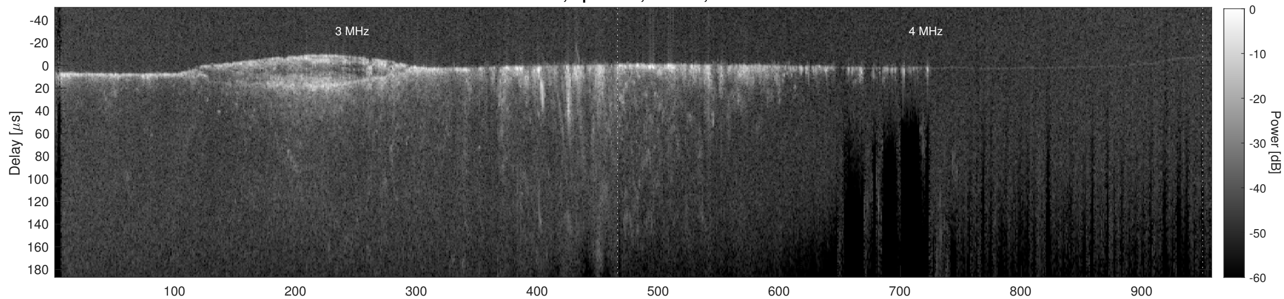
Orbit 13794, Cluttergram
