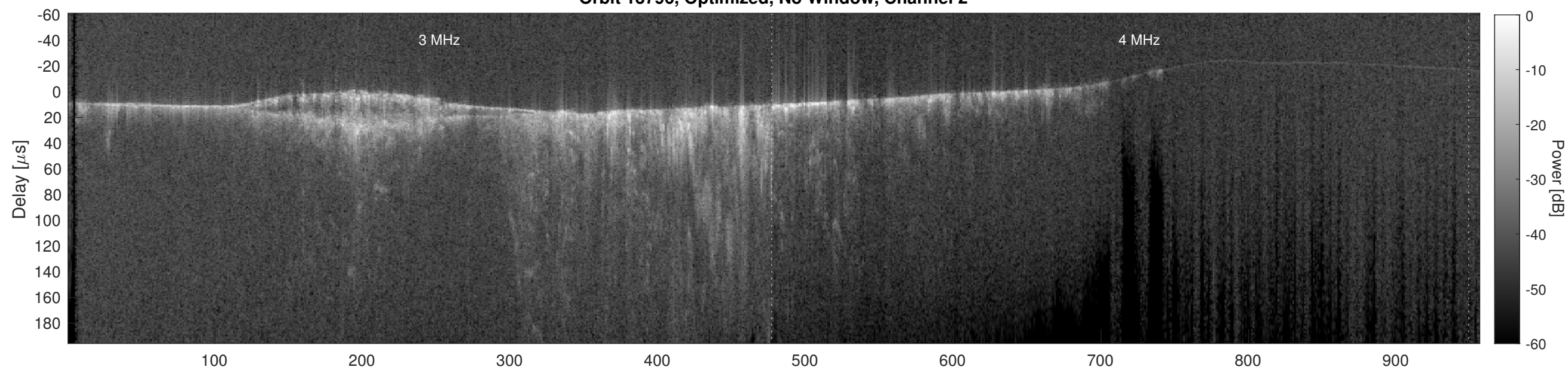
Orbit 13796, Cluttergram
