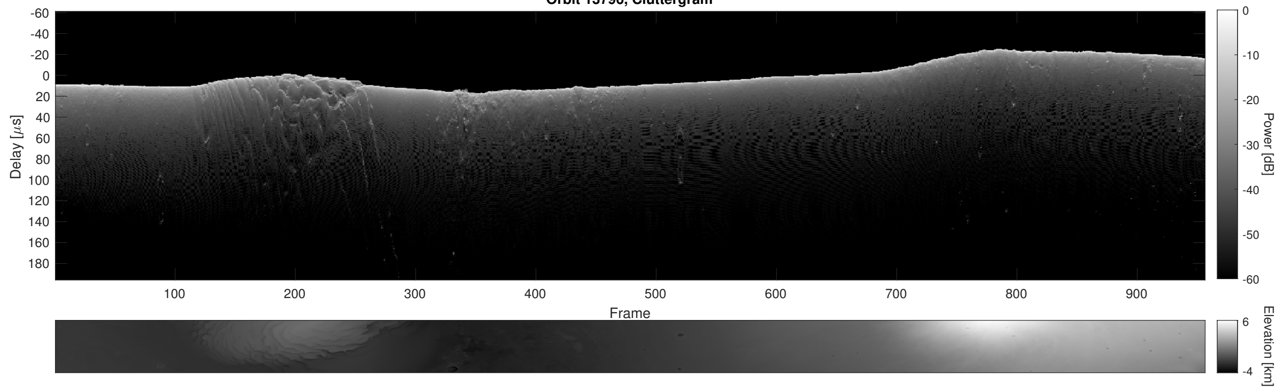
Orbit 13796, Cluttergram
