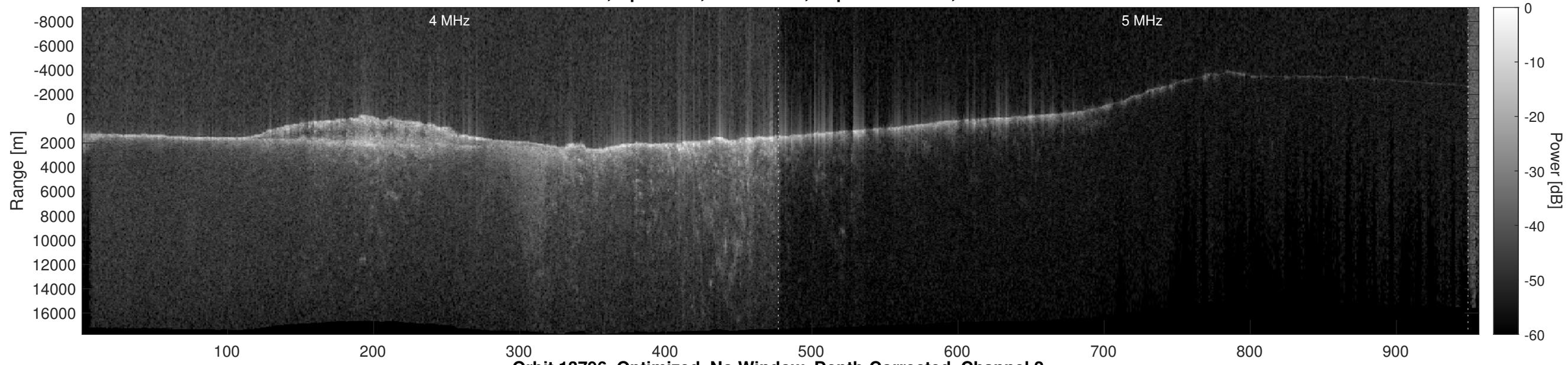
Orbit 13796, Optimized, No Window, Depth-Corrected, Channel 2
