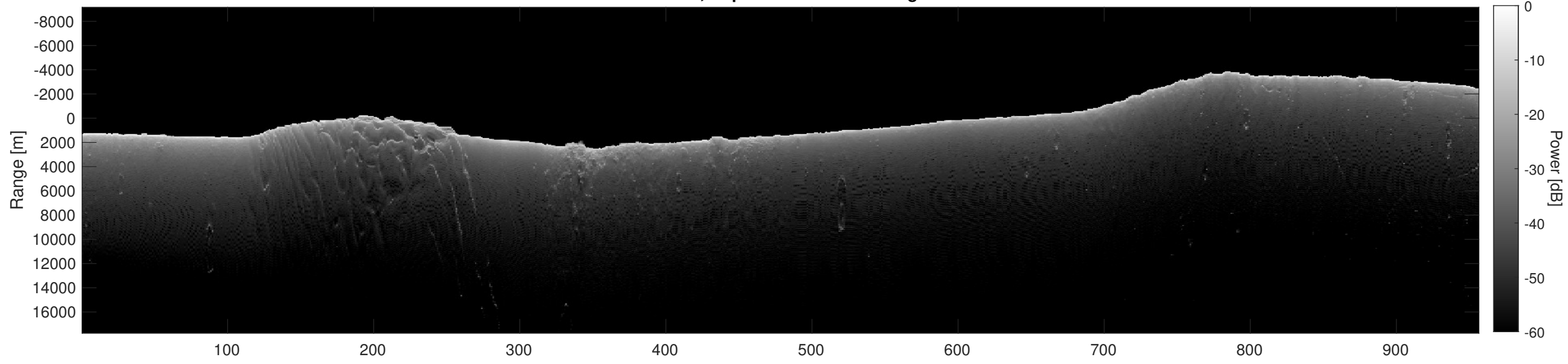
Orbit 13796, Depth-Corrected Cluttergram
