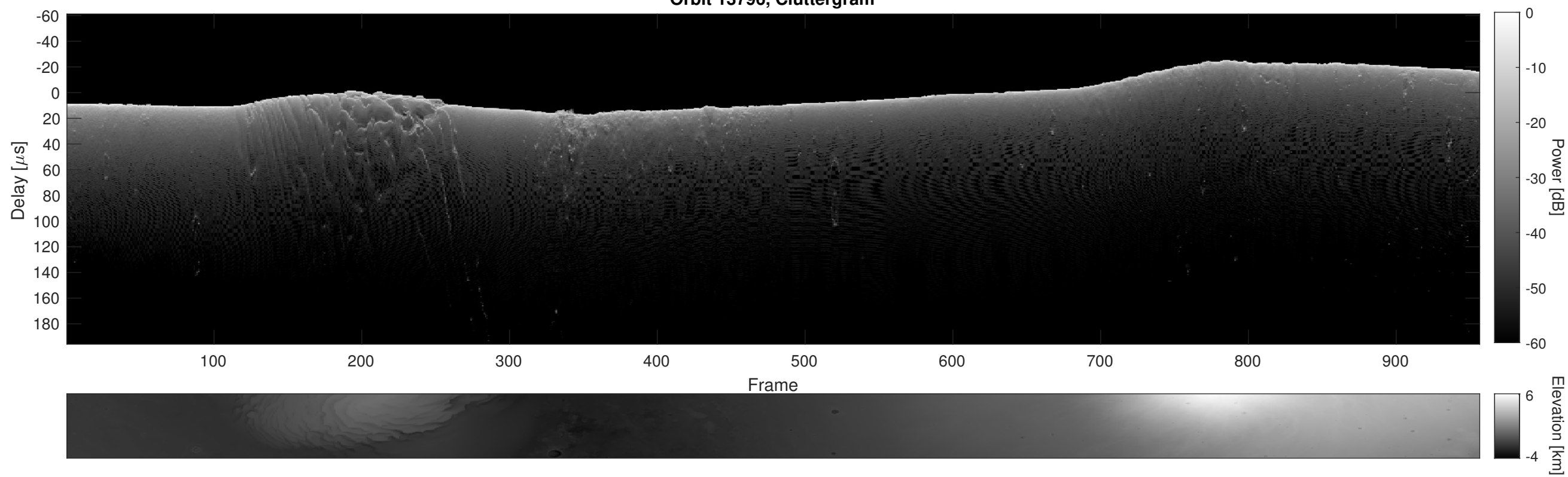
Orbit 13796, Cluttergram
