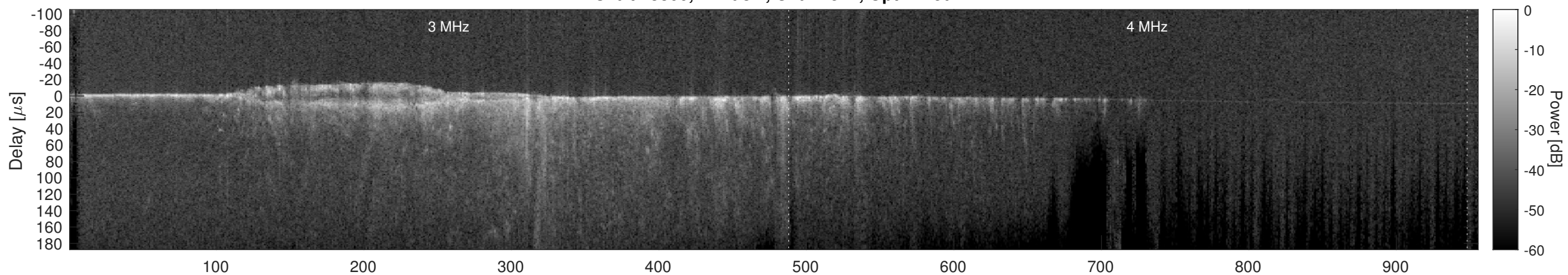
Orbit 13800, Cluttergram
