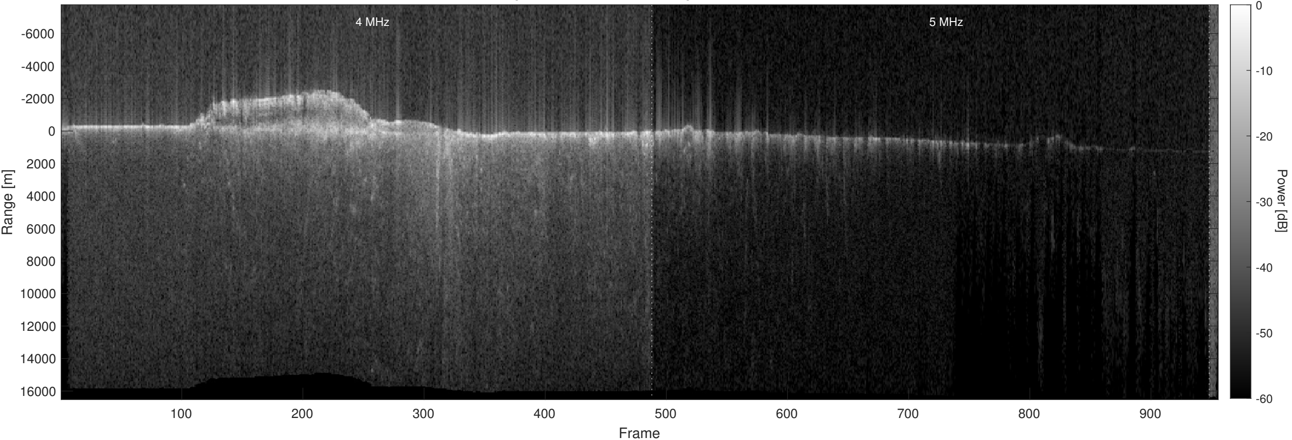
Orbit 13800, Optimized, No Window, Depth-Corrected, Channel 2
