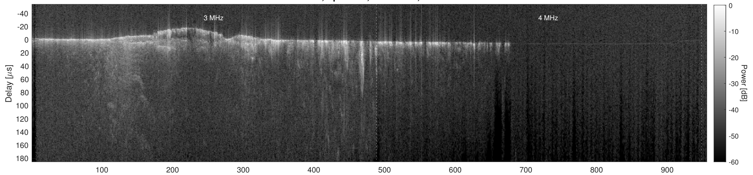
Orbit 13802, Cluttergram
