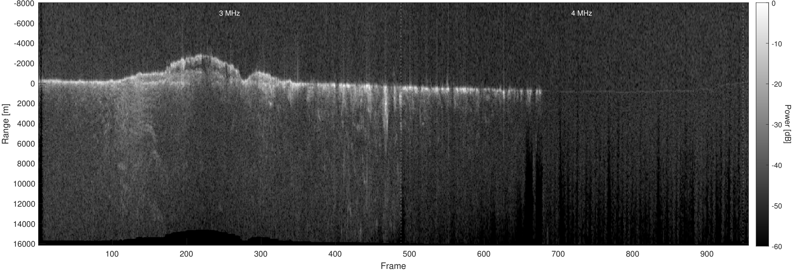
Orbit 13802, Optimized, Window, Depth-Corrected, Channel 2
