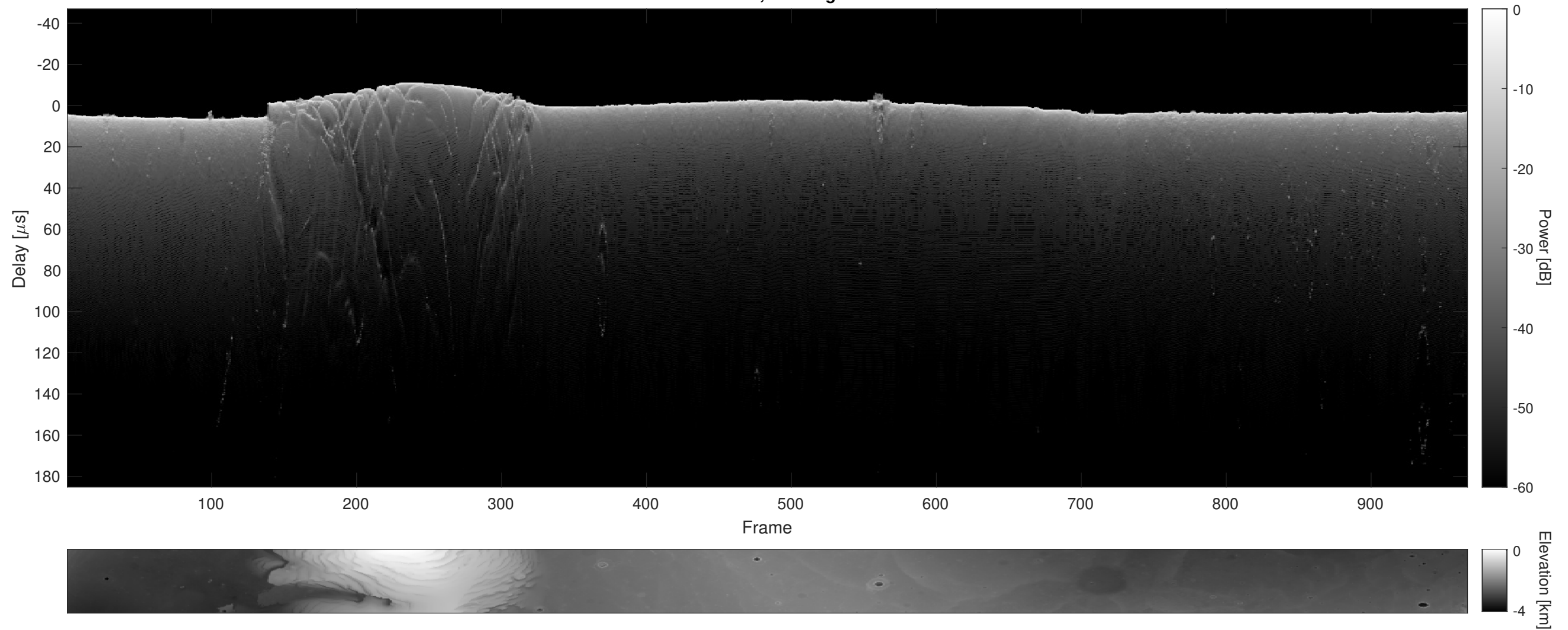
Orbit 13808, Cluttergram
