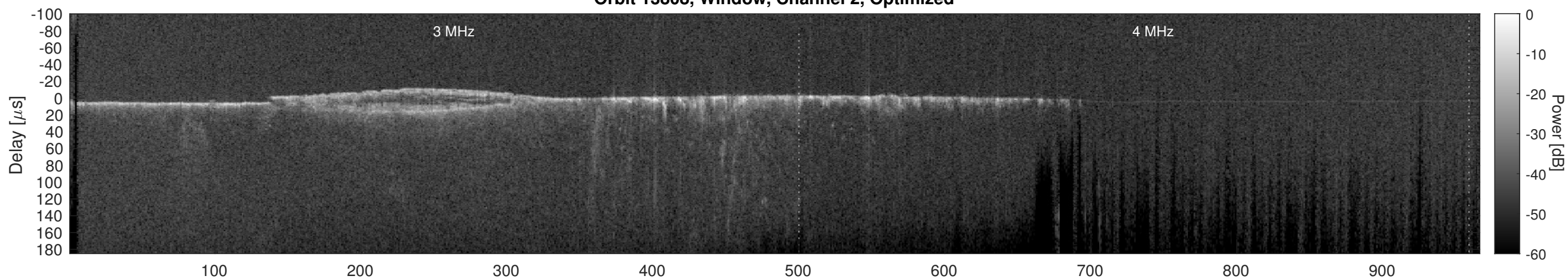
Orbit 13808, Cluttergram
