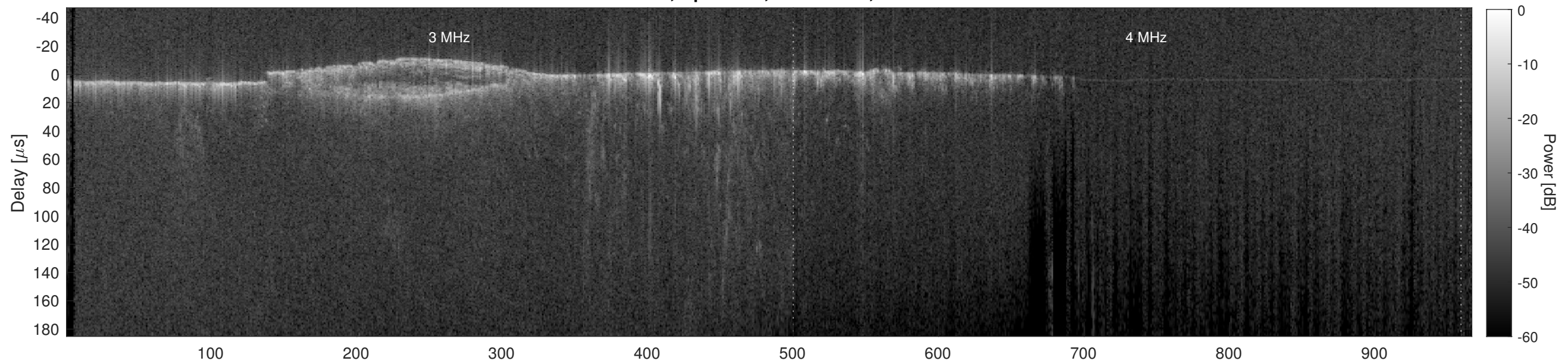
Orbit 13808, Cluttergram
