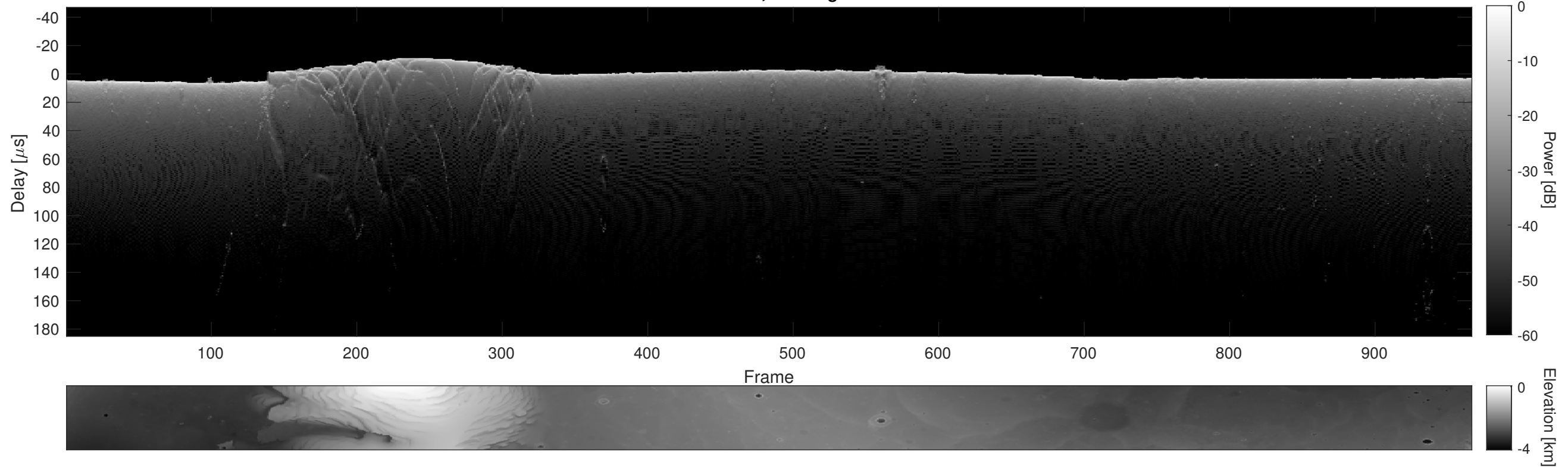
Orbit 13808, Cluttergram
