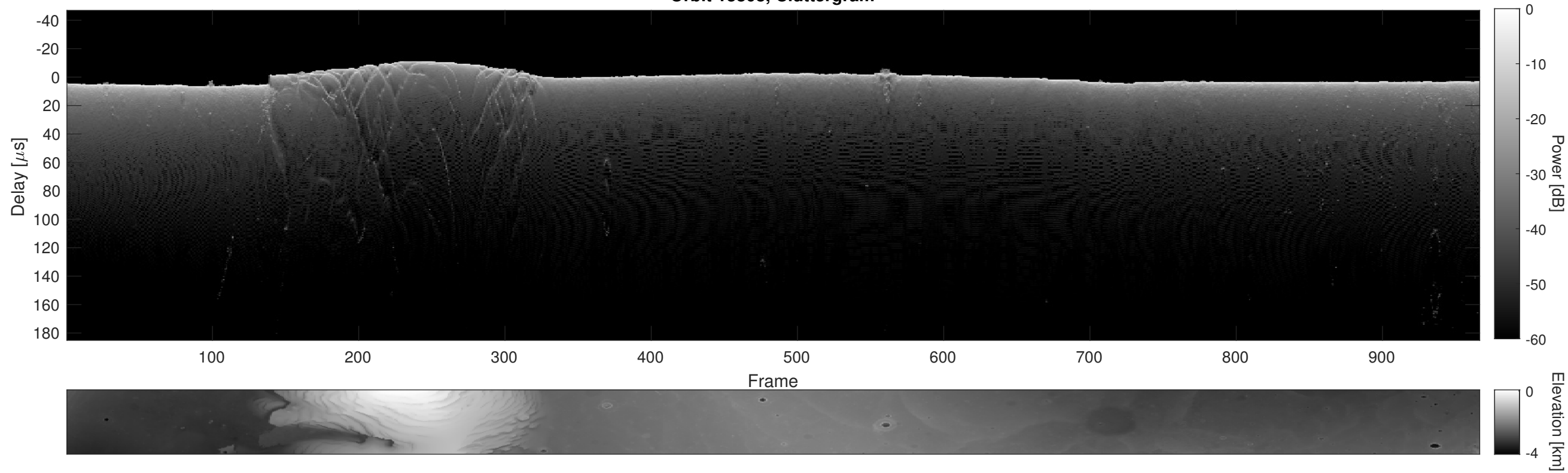
Orbit 13808, Cluttergram
