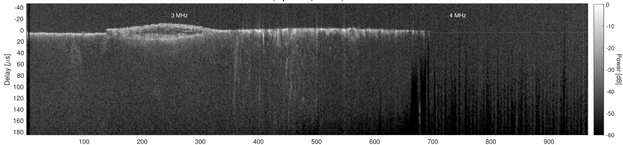
Orbit 13808, Cluttergram
