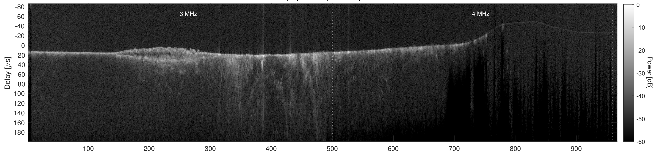
Orbit 13810, Cluttergram
