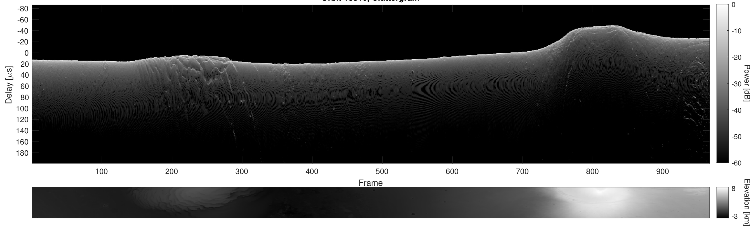
Orbit 13810, Cluttergram
