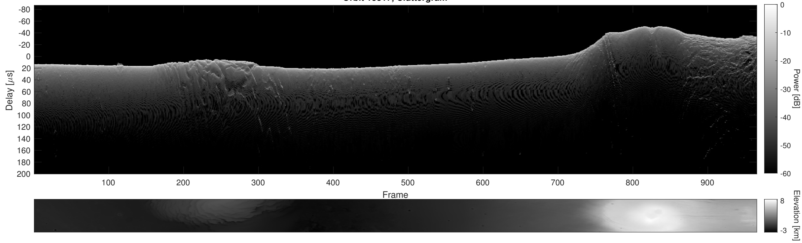
Orbit 13817, Cluttergram
