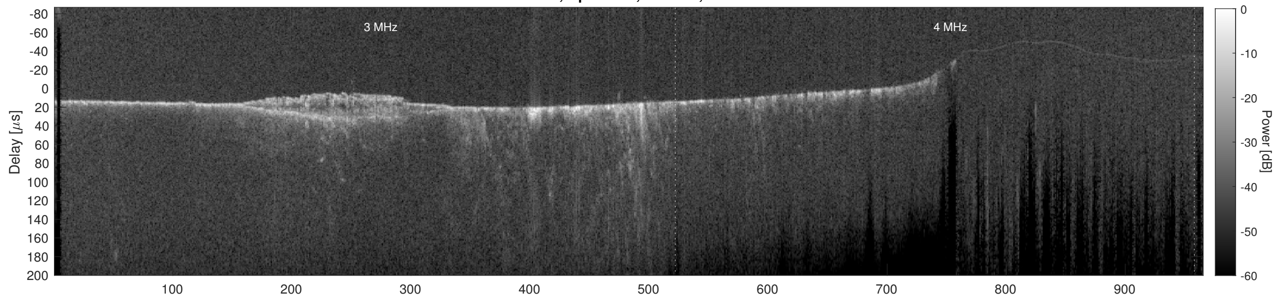
Orbit 13817, Cluttergram
