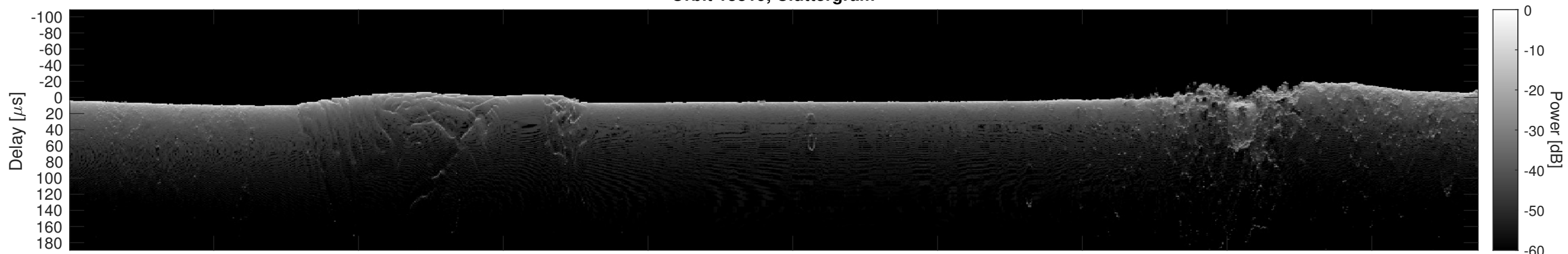
Orbit 13819, Cluttergram
