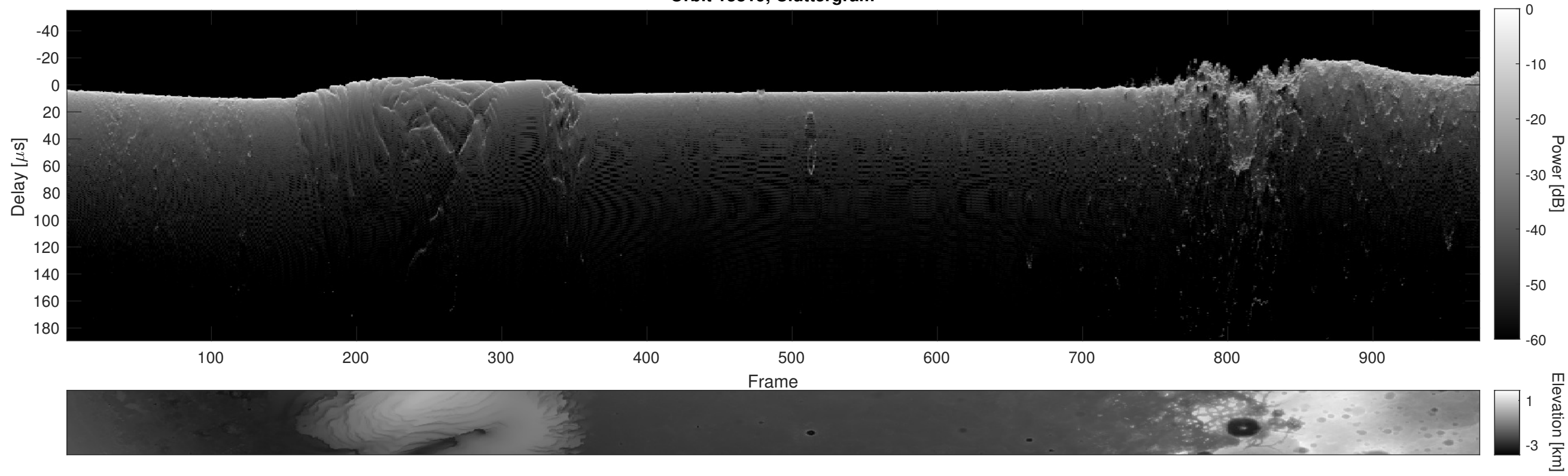
Orbit 13819, Cluttergram
