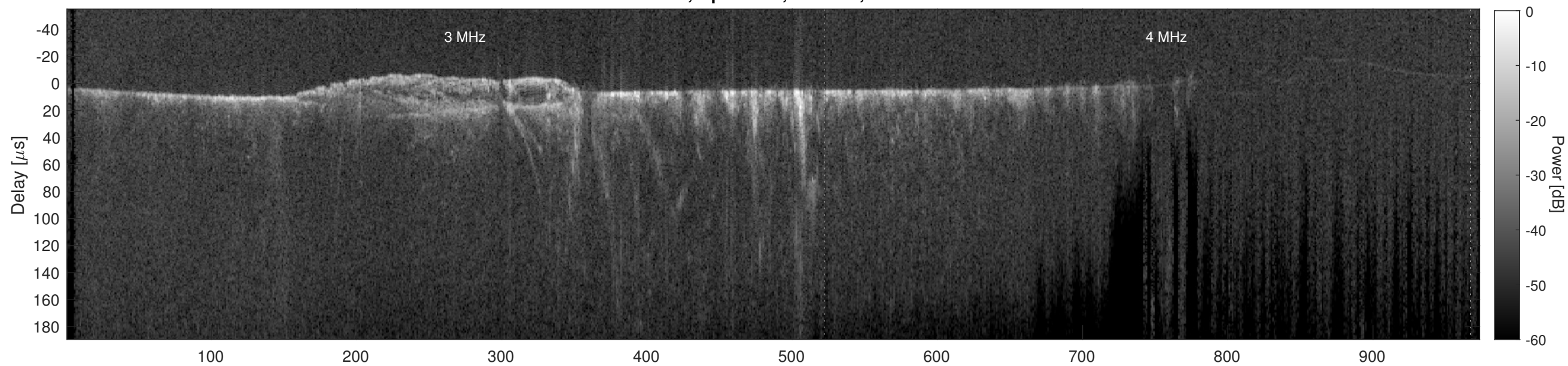
Orbit 13819, Cluttergram
